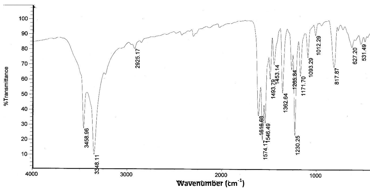
Figure S.1. FT-IR spectra of compound (2Z,4E)-3-(3,4-dihydroxyphenyl)-1,5-bis(2,4-dinitrophenyl) formazon (DPBDF)
