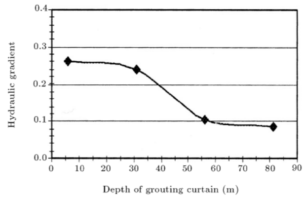
Figure 20. Variation of downstream toe gradient with grouting curtain depth.
