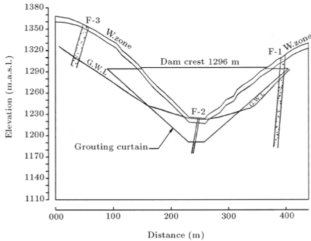
Figure 4. Longitudinal section of the dam (from upstream).
