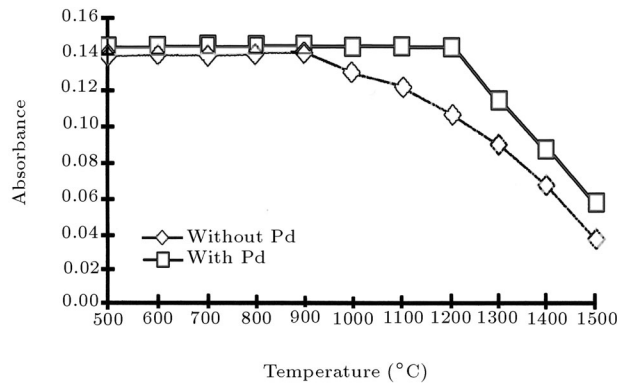
Figure 3. Pyrolysis curves for 10 ppb Mn, with 100 ppm Pd and without Pd in a solution containing 0.15 M NaCl and 3% HNO 3 .
