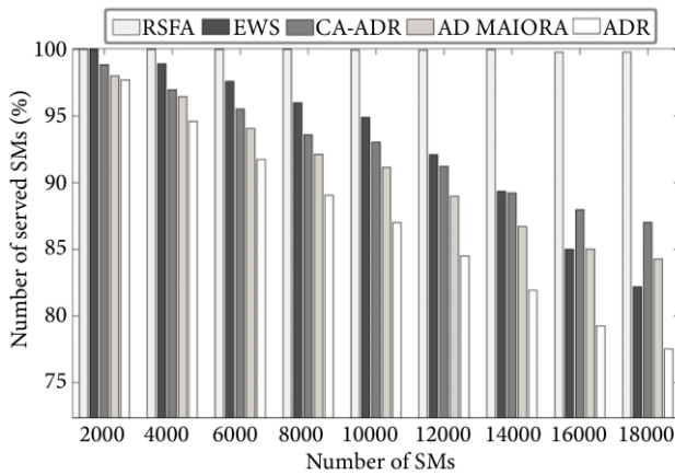
Figure 6. The ratio of the number of served SMs to the total number of SMs.
