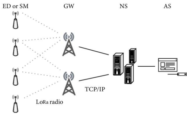
Figure 1. LoRaWAN architecture.
