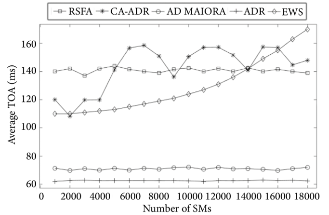
Figure 5. The average ToA for different numbers of SMs.
