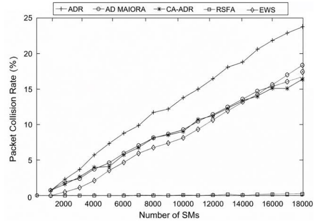
Figure 4. Packet collision rate for different numbers of SMs.
