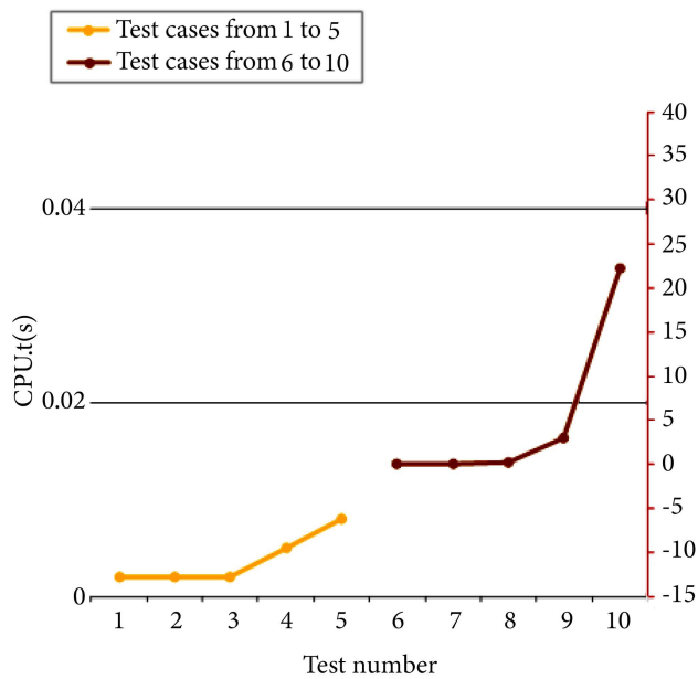
Figure 2. Computational time of the test cases solved by greedy heuristic algorithm (both vertical axes show CPU.t (s). the one on the left-hand side shows CPU.t of test Cases 1–5, and the one on the right-hand side shows that of test Cases 6–10.
