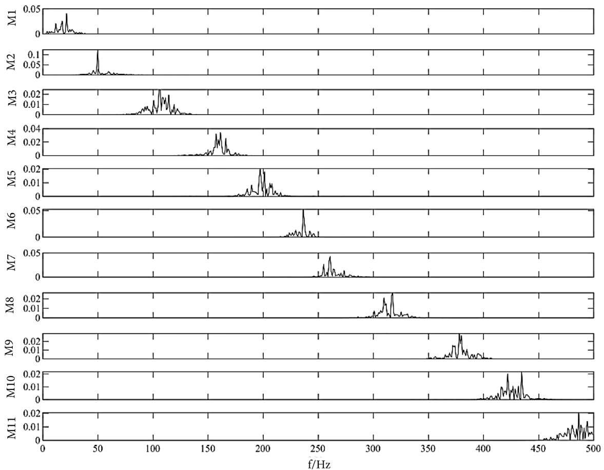
Figure 4. The spectrum of each component of VMD decomposition of 3 # oil sample.
