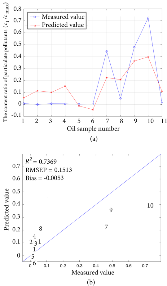
Figure 8. The comparison of the model-predicted value and measured value of full frequency spectrum.
