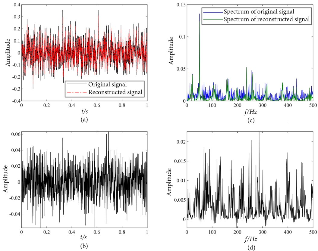
Figure 5. Comparison of original pressure signal and spectrum with the reconstructed signal of 3 # oil sample: (a) Comparison of the original signal with the reconstructed signal; (b) The error of original signal with the reconstructed signal; (c) Spectrum comparison of the original signal with the reconstructed signal; (d) Spectrum error of original signal with the reconstructed signal.
