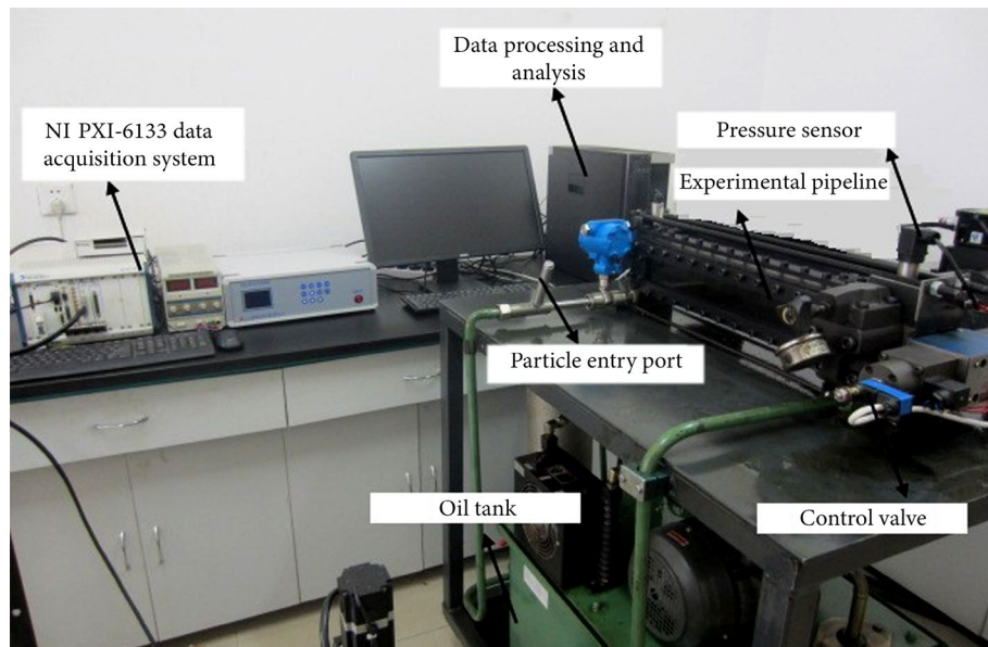
Figure 1. The experimental apparatus of the pressure vibration signal of the oil sample.
