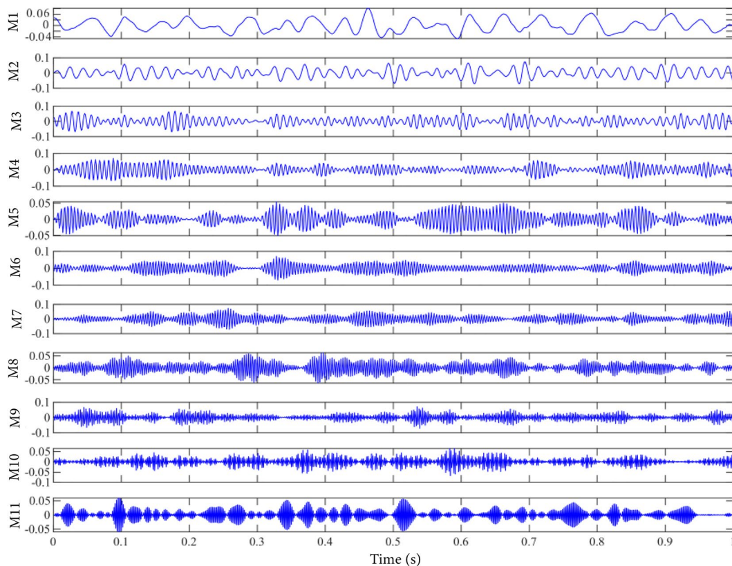
Figure 3. Components of the VMD decomposition of the 3 rd oil sample.
