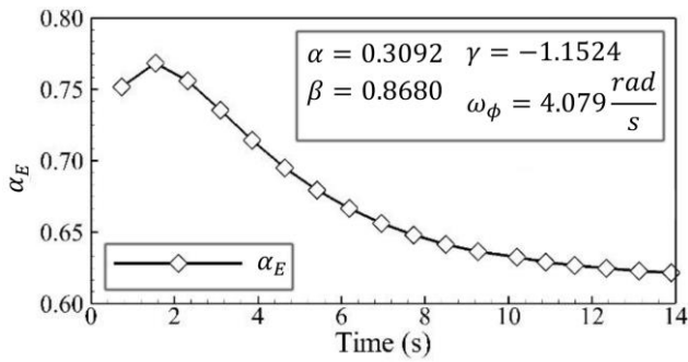
Figure 5. Equivalent linear damping coefficient ( T_S = 0.001 s).
