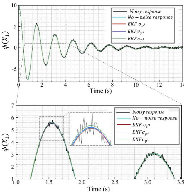
Figure 8. Comparison of actual and estimated roll angle for Scenario (b).
