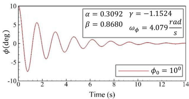
Figure 3. Simulated free roll decay with an initial angle \phi_0 = 10^\circ at Fr = 0.417 by running the fourth-order Runge-Kutta algorithm ( T_S = 0.001 s).
