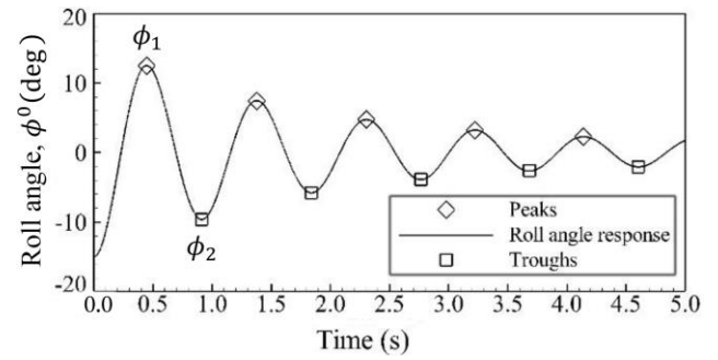
Figure 1. Typical roll decay curve.
