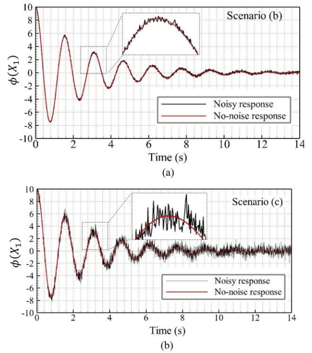
Figure 6. The simulated noisy signals ( T_S = 0.001 s). (a) \sigma_{m2} = 1 \times 10^{-2} deg; (b) \sigma_{m3} = 0.5 \times 10^{-1} deg.
