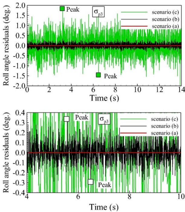
Figure 13. Residuals from EKF(s).
