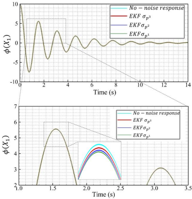
Figure 7. Comparison of actual and estimated roll angle for Scenario (a) (noiseless input).
