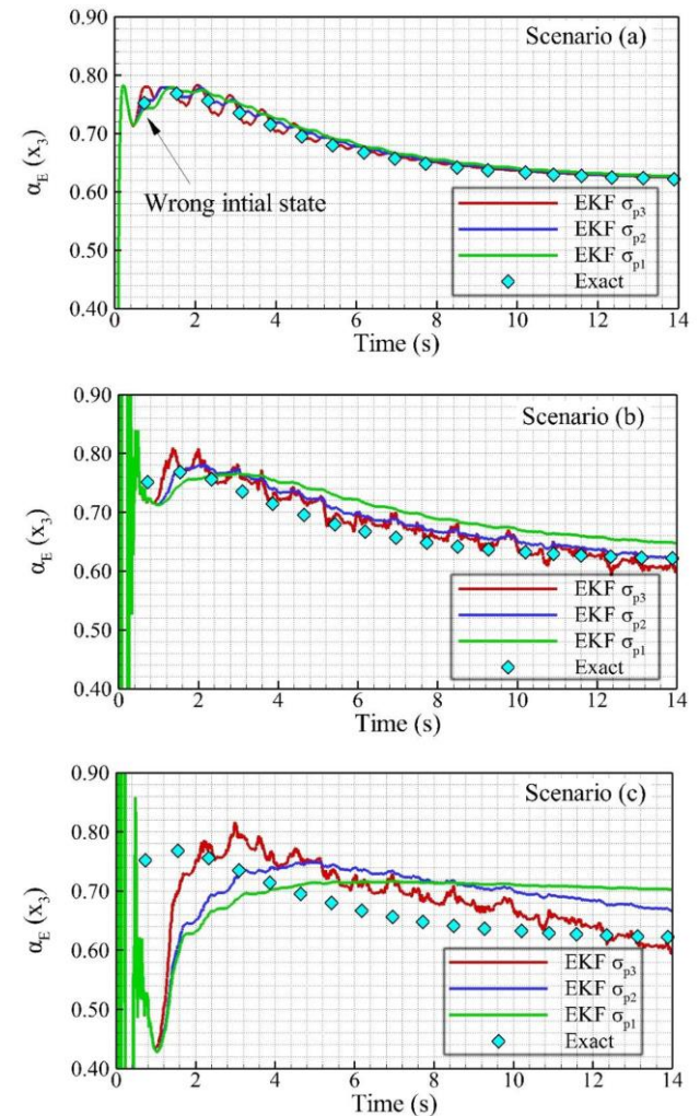
Figure 11. The estimated value of equivalent linear damping coefficient ( \alpha_E ) for three scenarios.
