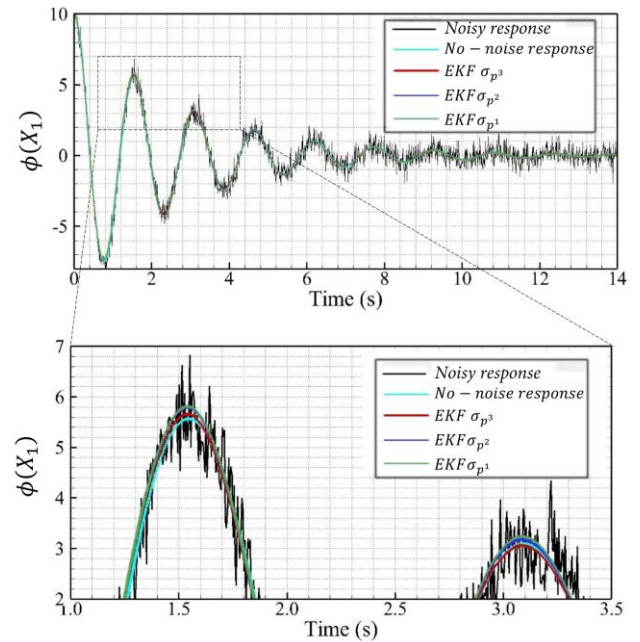
Figure 9. Comparison of actual and estimated roll angle for Scenario (c). Table 5. RMSE values for the first state for various choices of \sigma_{p3} in EKF(s).
