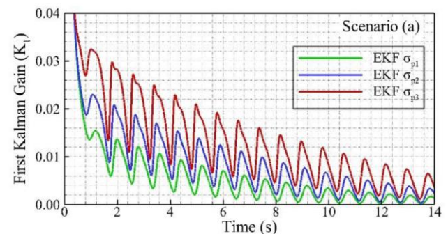
Figure 12. The effects of process-noise covariance matrix Q on the Kalman gain.
