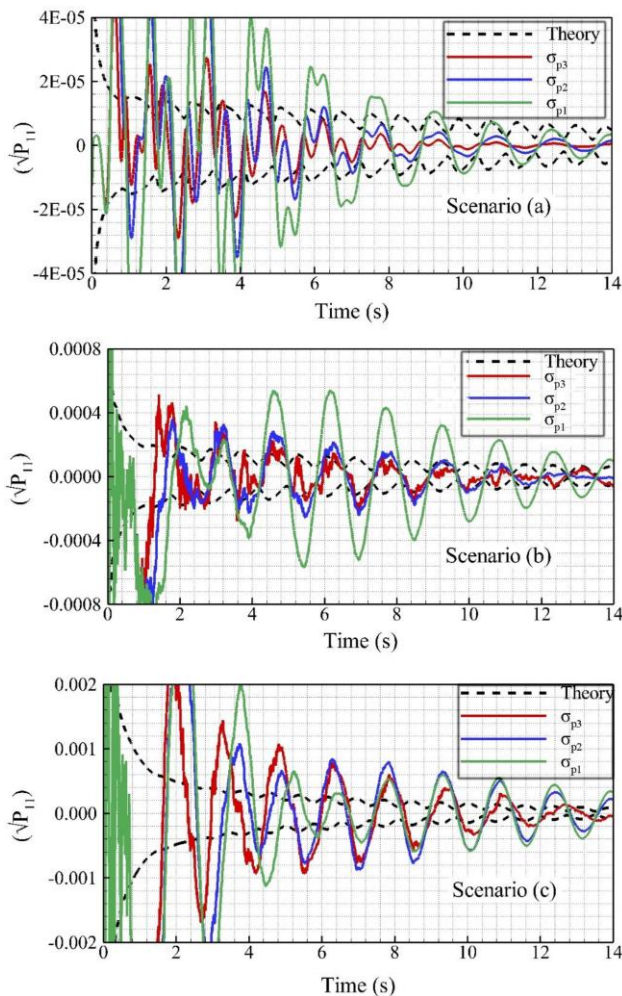
Figure 10. Covariance propagation of the \phi(x_1) for three simulation scenarios.
