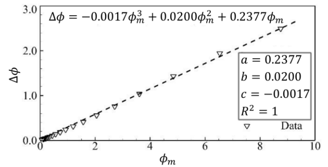
Figure 4. Extinction curve ( T_S = 0.001 s).
