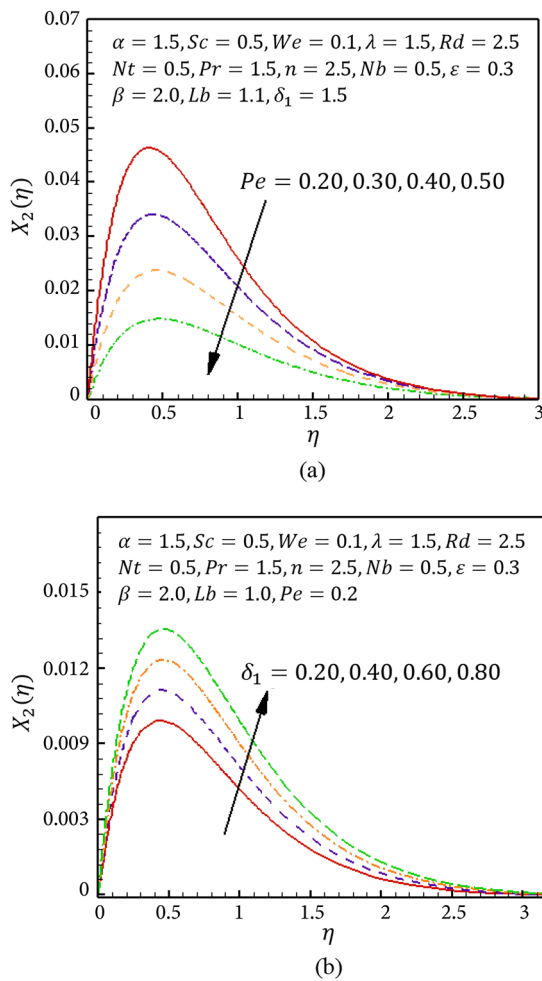
Figure 10. Consequences of [Pe] and [\delta_1] on \chi_2(\eta) .
