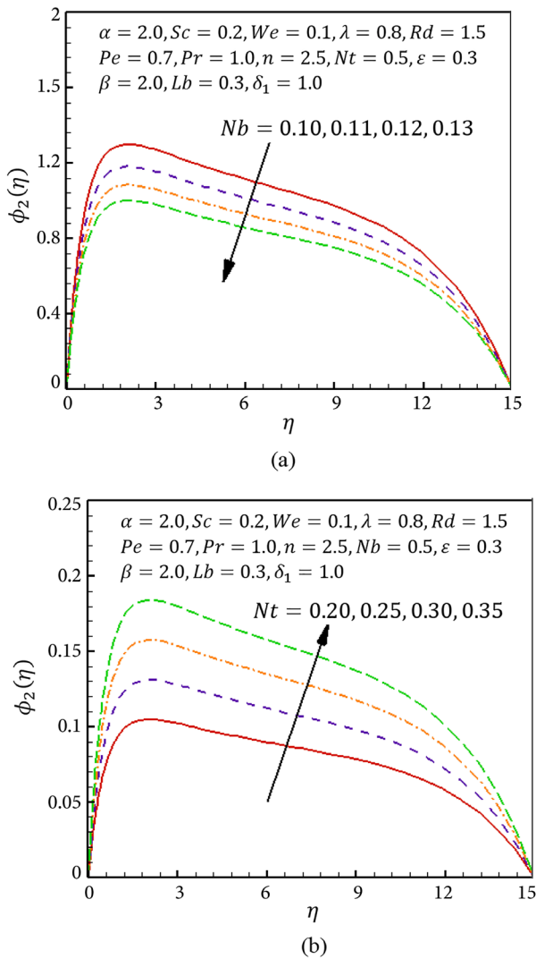
Figure 8. Impact of different [N_b] and [N_t] on \phi_2(\eta) .
