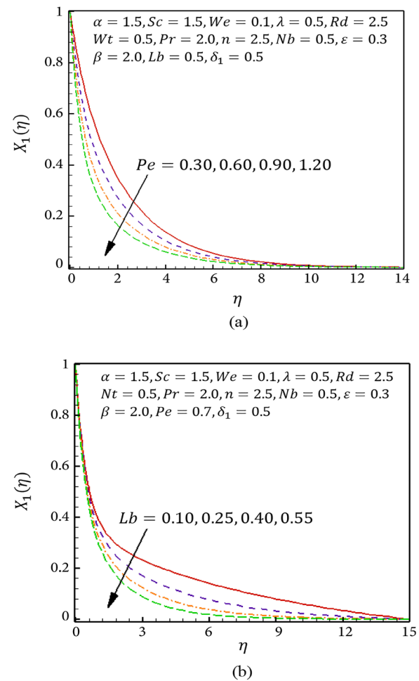
Figure 9. Consequences of [Pe] and [Lb] on \chi_1(\eta) .
