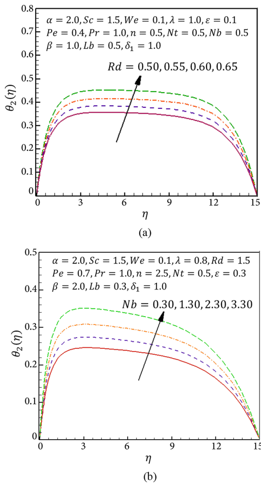
Figure 6. Aspects of different values of [Rd] and [Nb] against \theta_2(\eta) .
