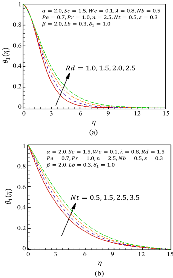
Figure 4. Impression of dissimilar estimations of [Rd] and [N_t] against \theta_1(\eta)
