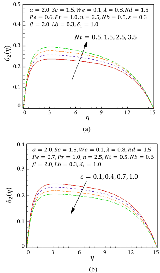
Figure 5. Impact of different values of [N_t] and [\varepsilon] on \theta_2(\eta) .
