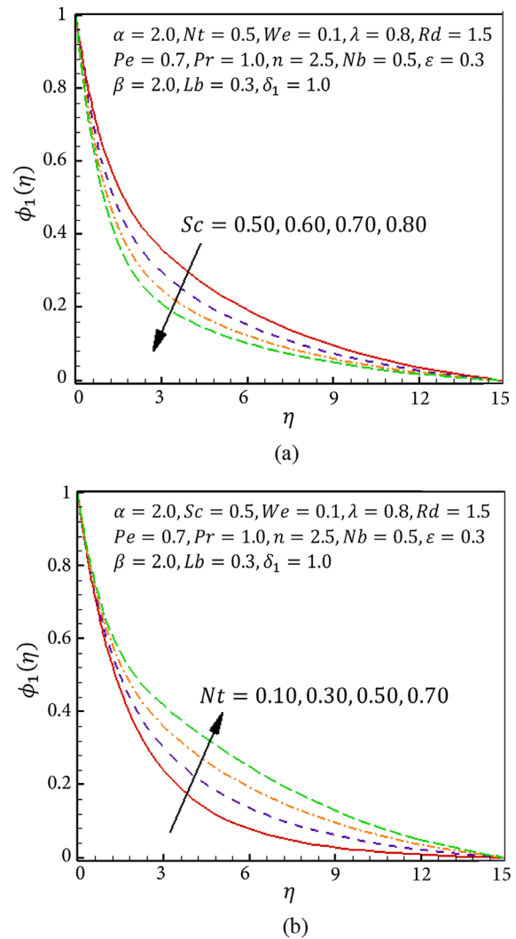
Figure 7. Influence of diverse effected [Sc] and [Nt] on \phi_1(\eta) .
