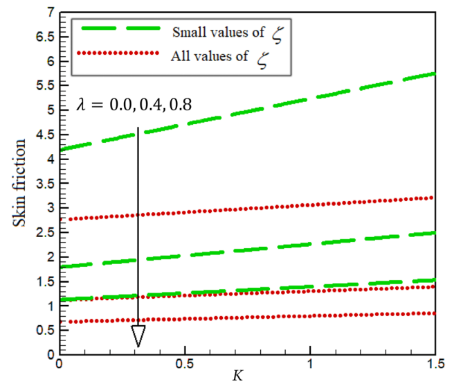
Figure 6. Comparative results of \lambda and K for skin friction.
