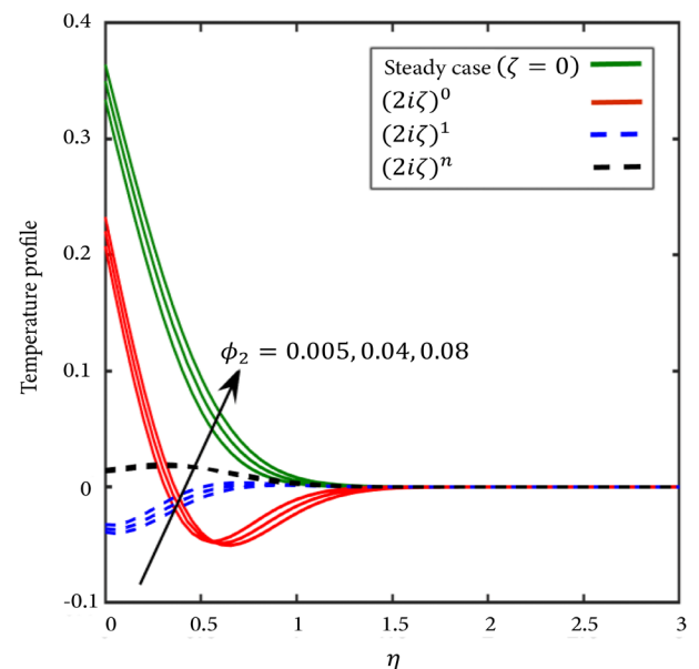
Figure 2. Difference between temperature and \Phi_2 .
