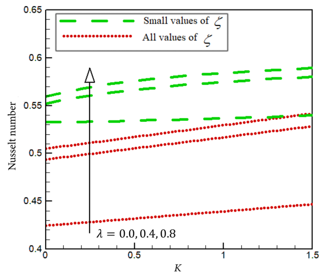
Figure 7. Comparative results of \lambda and K for Nusselt number.
