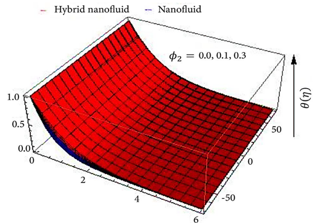
Figure 13. Influence of \phi_2 via with temperature field.
