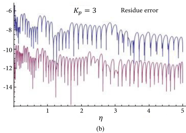
Figure 3. Error estimation for K_p = 3 .
