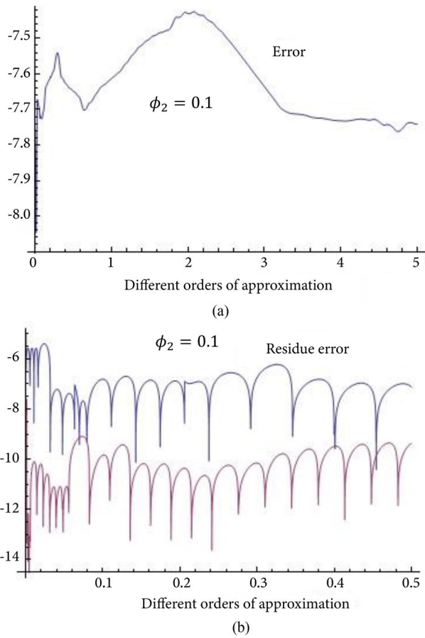
Figure 7. Error estimation for \phi_2 = 0.1 .
