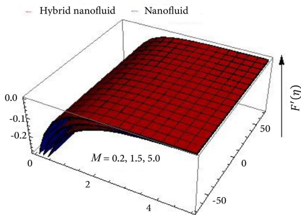
Figure 17. Influence of M via velocity field.
