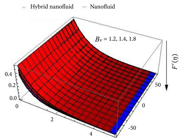
Figure 18. Influence of B_v via Dust Phase Velocity (DPV).
