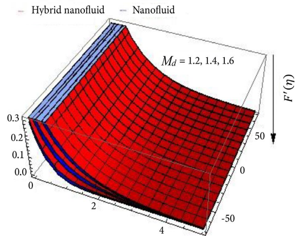
Figure 19. Influence of M_d via Dust Phase Velocity (DPV).
