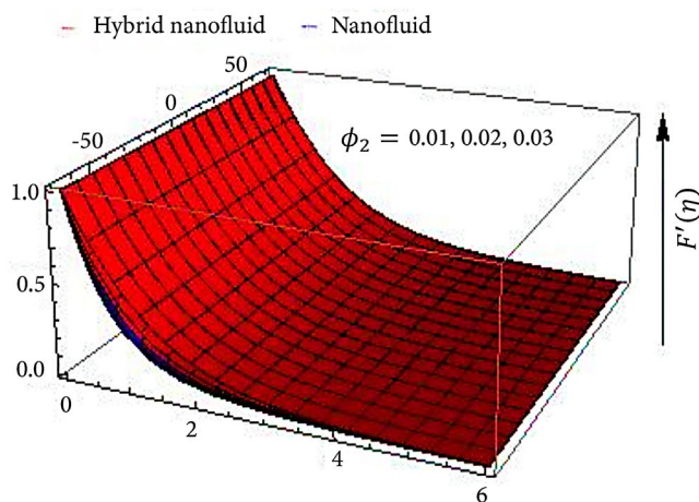
Figure 12. Influence of \phi_2 via Dust Phase Velocity (DPV).
