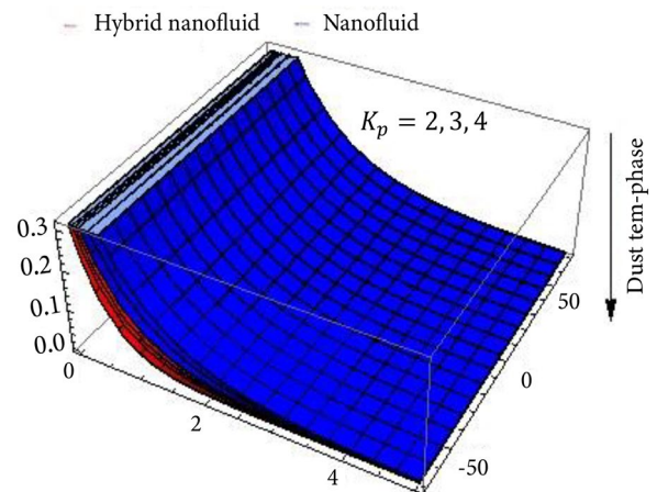
Figure 10. Motivation of K_p via DPT.
