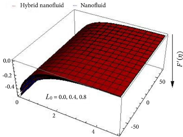
Figure 15. Influence of L_0 via with velocity field.
