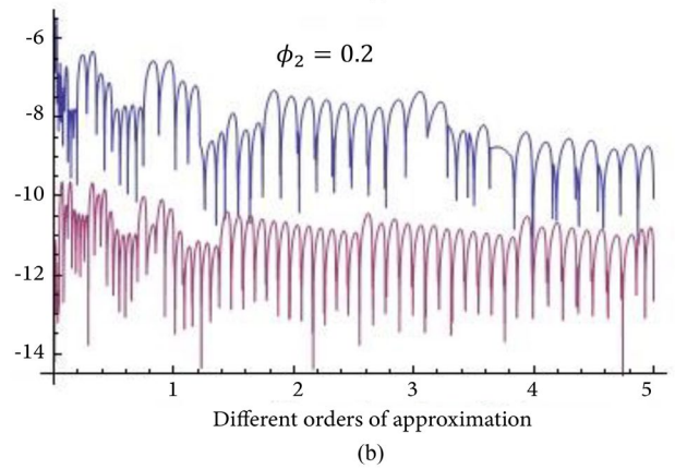
Figure 5. Error estimation for \phi_2 = 0.2 .
