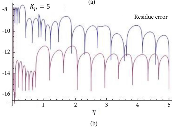
Figure 4. Error estimation for K_p = 5 .
