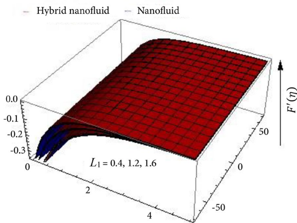
Figure 16. Influence of L_1 via velocity field.
