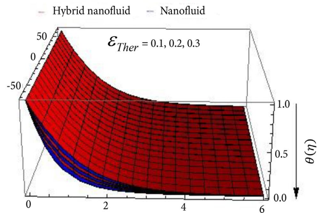
Figure 20. Influence of \mathcal{E}_{Ther} via temperature field.
