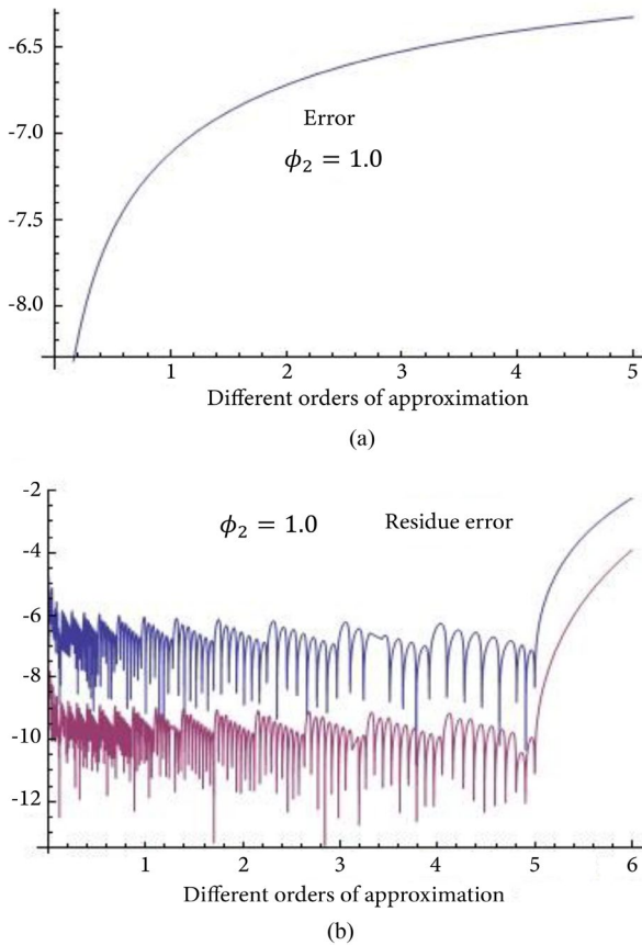
Figure 8. Error estimation for \phi_2 = 1.0 .
