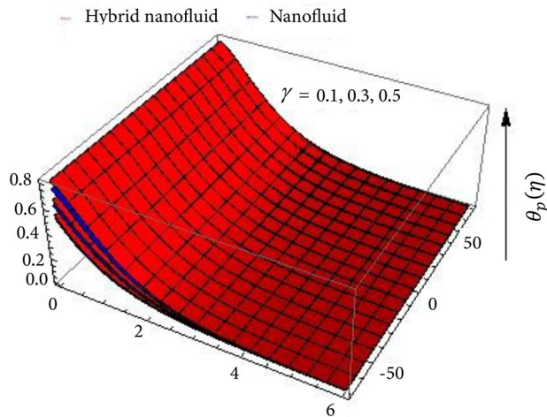
Figure 21. Influence of \gamma via DPT.
