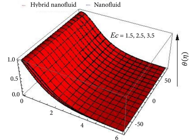
Figure 22. Influence of E_c via temperature field.
