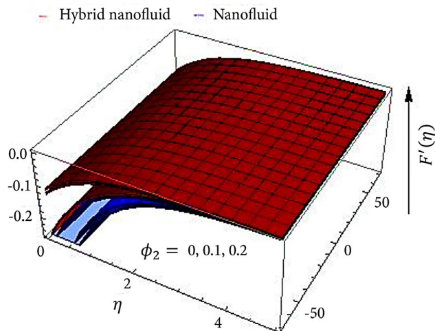
Figure 11. Influence of \phi_2 via velocity field.
