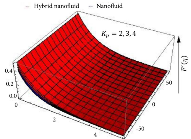
Figure 9. Motivation of K_p via Dust Phase Velocity (DPV).
