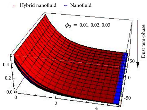
Figure 14. Influence of \phi_2 via DPT.
