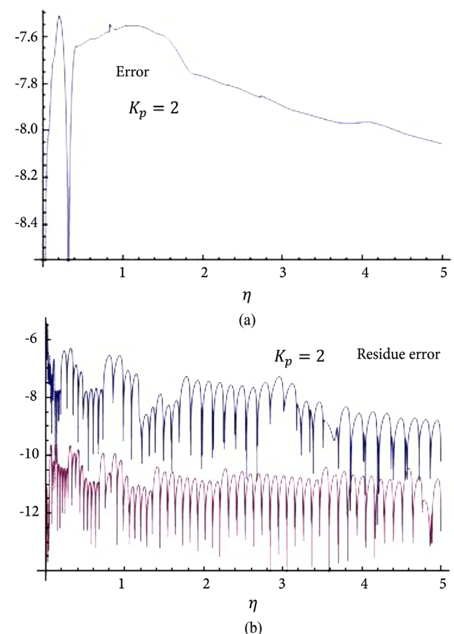
Figure 2. Error estimation for K_p = 2 .
