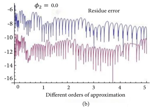
Figure 6. Error estimation for \phi_2 = 0.0 .
