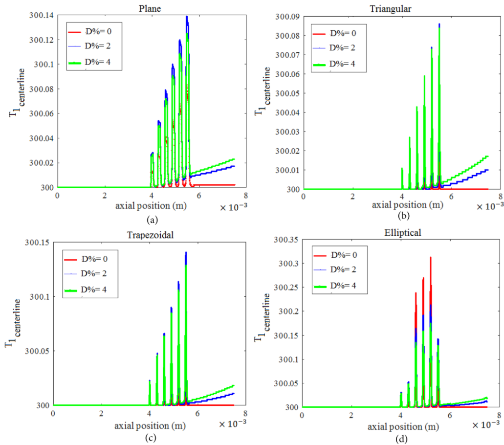
Figure 11. Variations of D\% vs. plots of T_{1\_centerline} at Re = 60 for (a) plane, (b) triangular, (c) trapezoidal, and (d) elliptical obstacle cases along the centerline.
