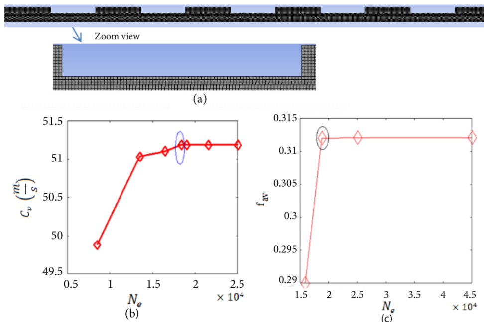
Figure 3. (a) Geometry of mesh configuration, variations of (b) C_v and (c) f_{av} versus N_e for D\% = 0 , at Re = 120 .
