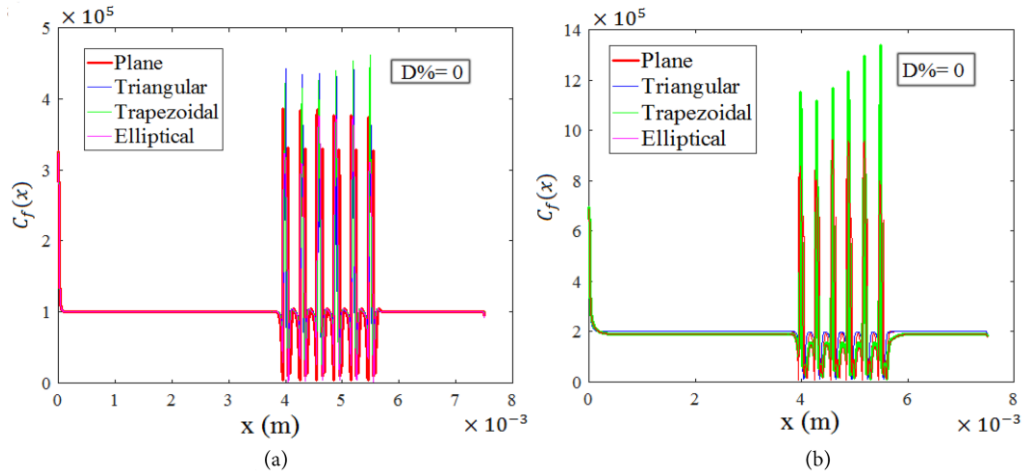
Figure 13. Plots of C_f(x) on the heated wall at Re = (a) 120, (b) 60 for various obstacle configurations.
