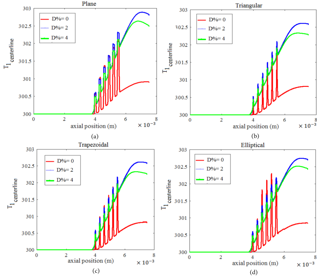
Figure 10. Variations of D\% vs. plots of T_{1\_centerline} at Re = 1 for (a) plane, (b) triangular, (c) trapezoidal, and (d) elliptical obstacle cases along the centerline.
