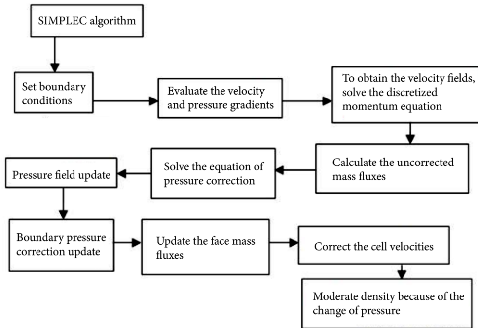
Figure 2. Working procedure of SIMPLEC algorithm.
