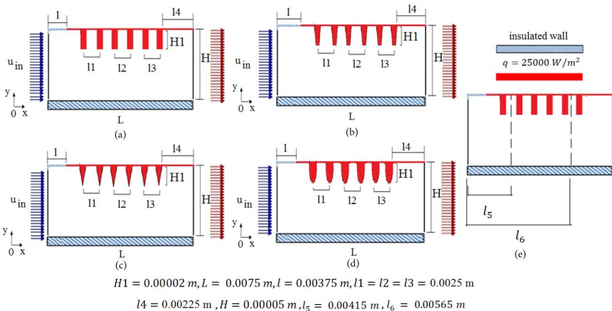
Figure 1. Rectangular channel embedded with (a) plane, (b) trapezoidal, (c) triangular, (d) elliptical obstacles, and (e) locations of generating plane.
