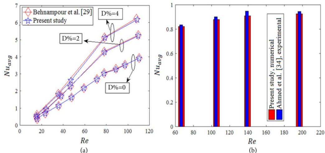
Figure 4. Validation of current study with (a) Behnampour et al. [29] (numerical work) and (b) Ahmed et al. [34] (experimental work) by analyzing the profiles of Nu_{avg} vs. Re .
