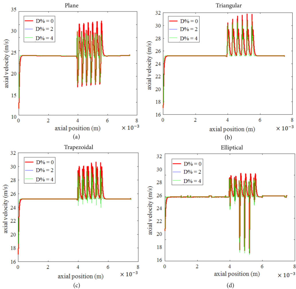
Figure 6. Variations of D\% vs. plots of axial velocity at Re = 60 for (a) plane, (b) triangular, (c) trapezoidal, and (d) elliptical obstacle cases along the centerline.
