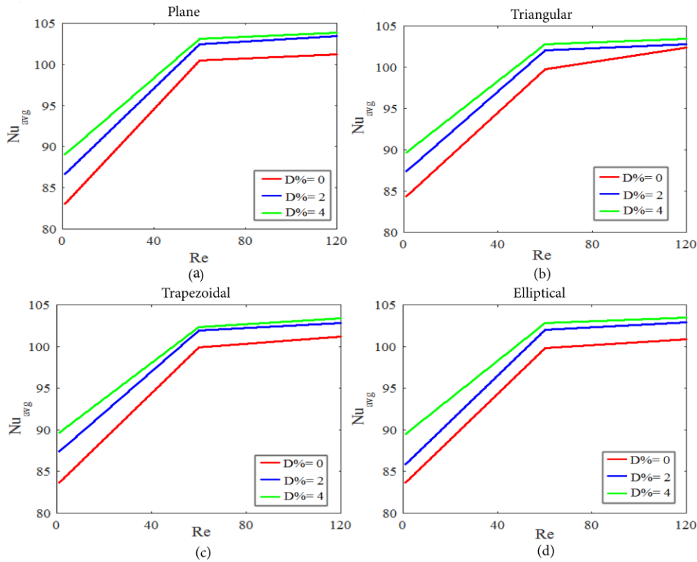
Figure 15. Plots of Nu_{avg} on the heated wall for various Re , and obstacle configurations.
