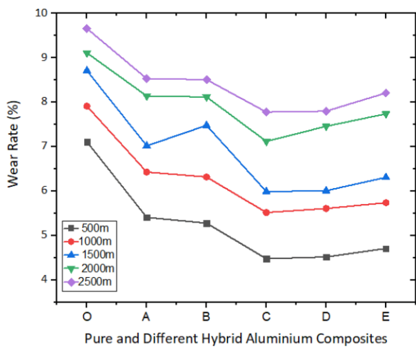
Figure 8. Wear rate of pure and hybrid composites at sliding distance variation.
