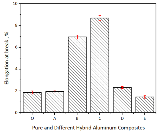
Figure 6. Elongation at break of all hybrid composites filled with V&Sn.
