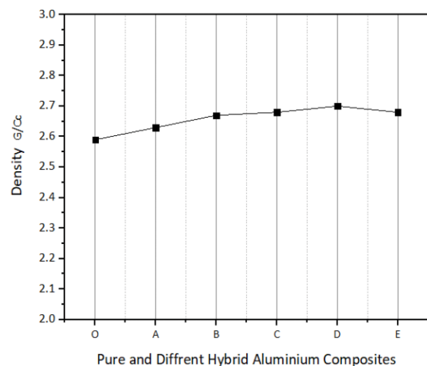
Figure 2. Density of all hybrid composites filled with V&Sn.
