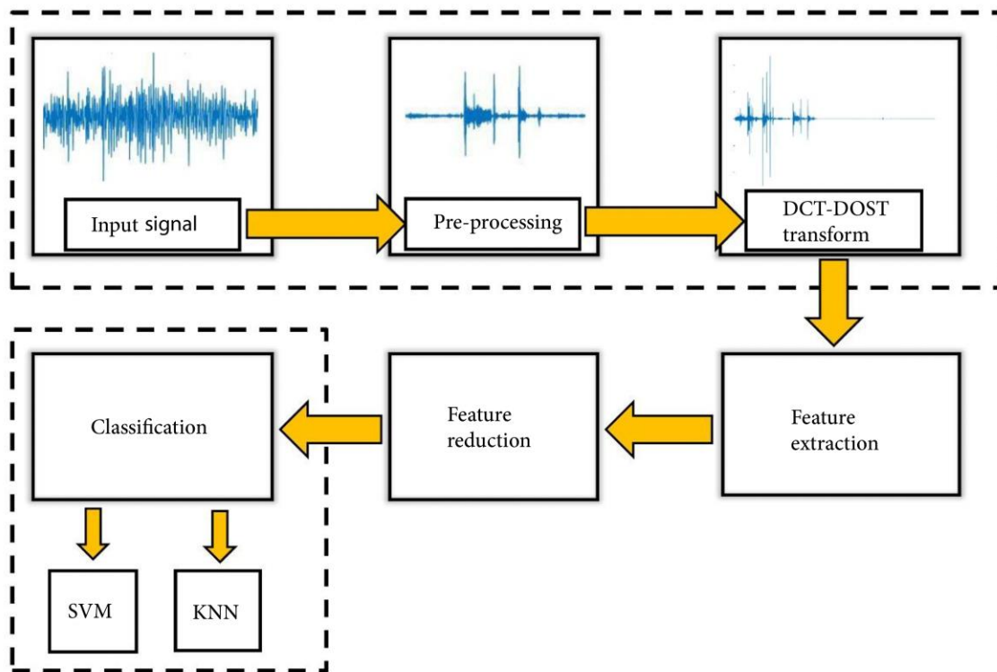
Figure 2. Block diagram of the proposed method.
