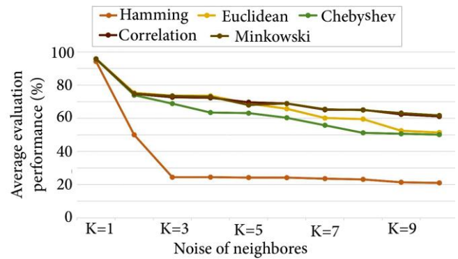
Figure 5. The average result (sensitivity, specificity, precision and accuracy) of five different distances for neighborhood numbers 1 to 10 with the KNN classifier.
