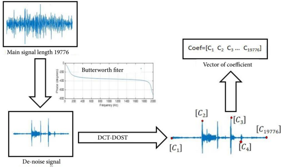
Figure 3. Block diagram of the DCT-DOST transform.
