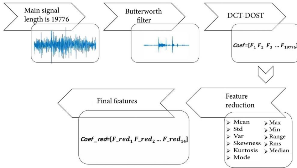
Figure 4. Schematic of feature reduction.
