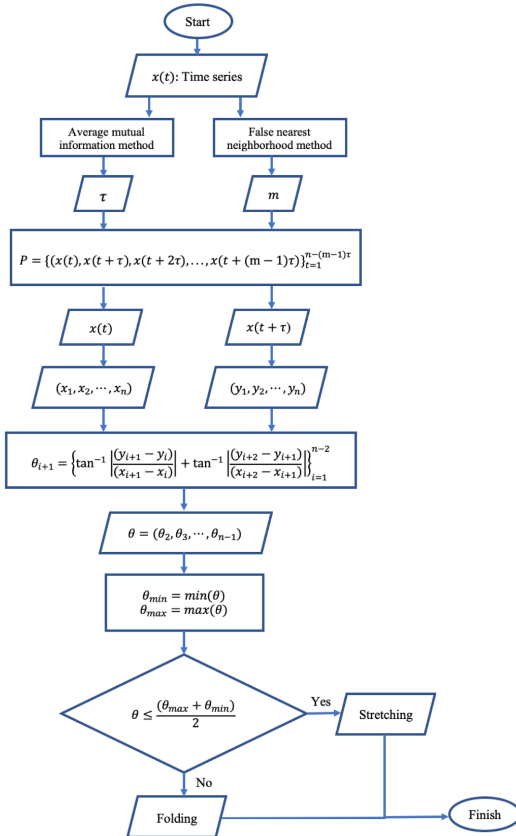
Figure 2. Flowchart of the proposed method, based on the SF definition, in which SF points are identified from variations in the trajectory's angle and/or slope at each phase-space point. High-slope points where the trajectory bends are classified as folding, whereas low-slope points where the trajectory changes rapidly over a large phase-space area are classified as stretching.
