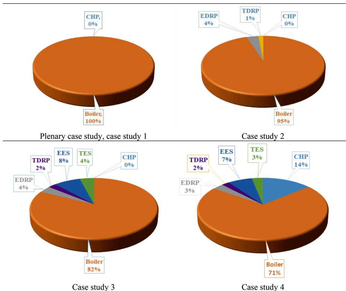
Figure 9. Share of flexible resources in EH flexibility provision.
