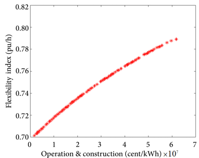
Figure 8. Pareto front of the problem under GPU.
