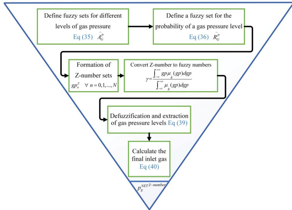
Figure 4. GPU modeling process using Z-number.
