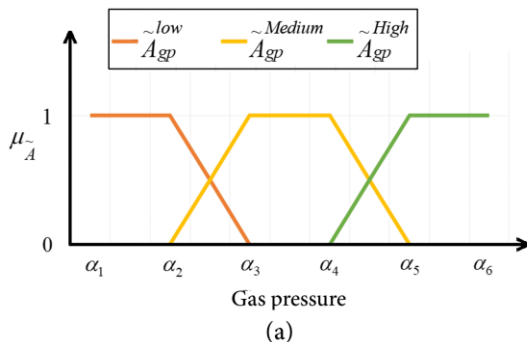
Figure 2. Gas pressure level (a) and probability modeling of gas pressure level (b) in the Z-number method.
