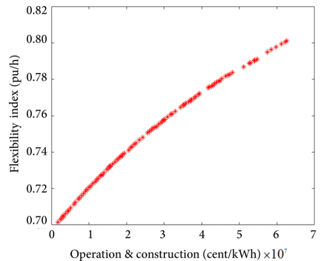
Figure 7. Pareto front of MOF-EH_{MC}^{soco} problem without GPU.
