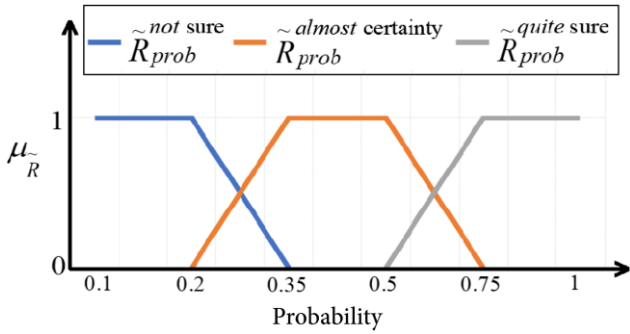
Figure 11. Defined Z-number probabilistic sets for gas pressure.
