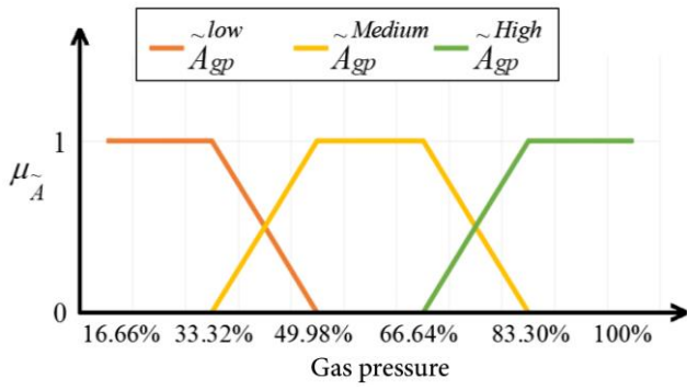
Figure 10. Defined Z-number fuzzy sets for gas pressure.
