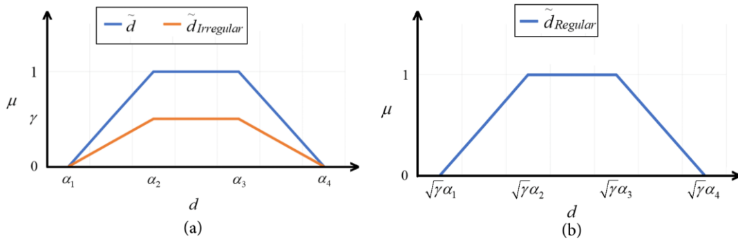
Figure 3. Regulation of the fuzzy number process.
