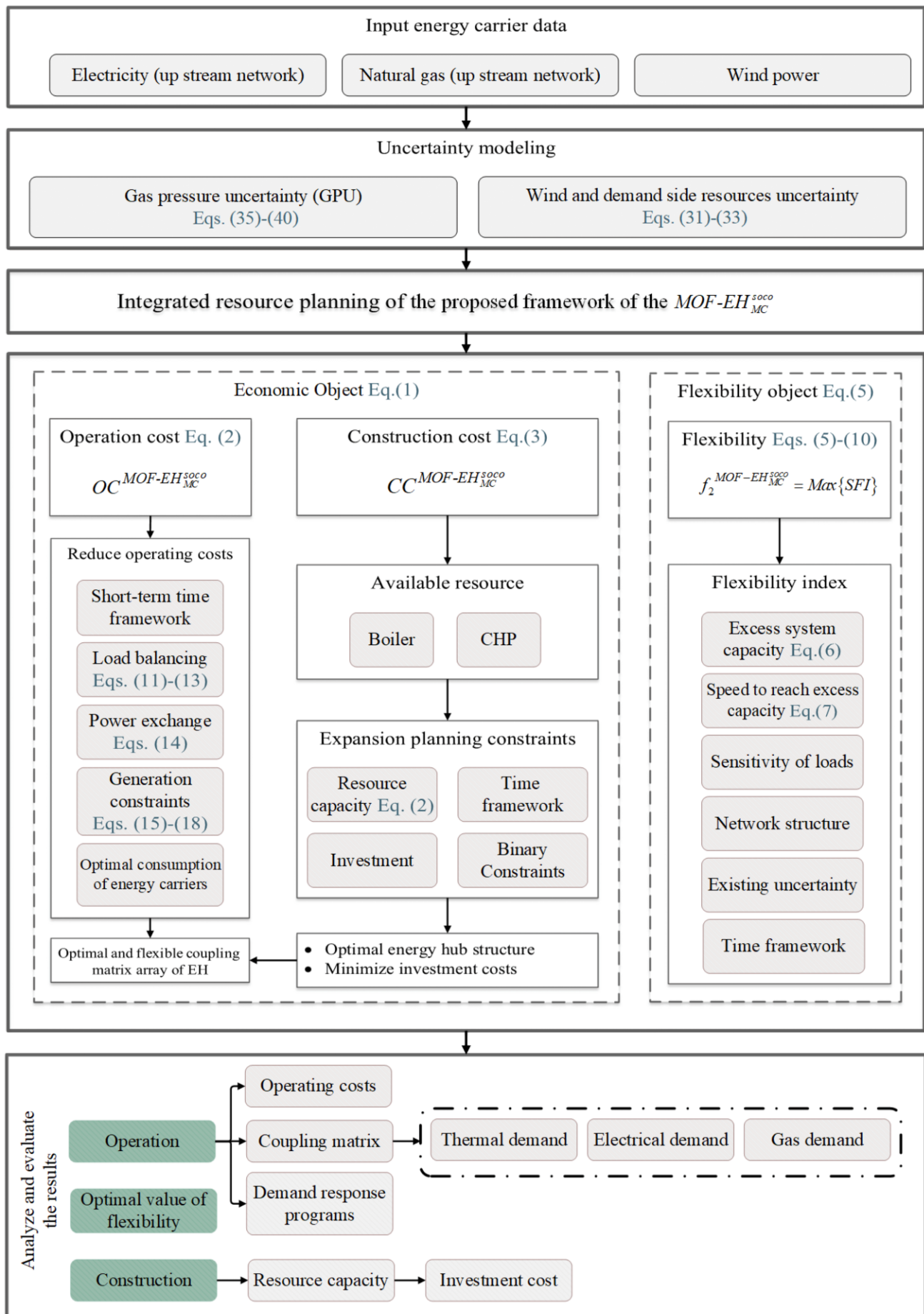
Figure 1. Framework of implementing proposed MOF-EH^{soco}_{MC} .
