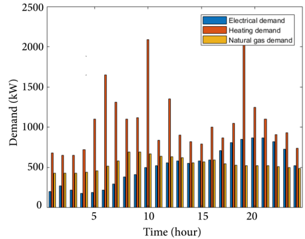
Figure 5. Thermal, electrical, and gas demand [33].
