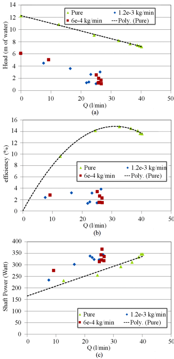
Figure 13. Experimental relation between (a) head, (b) efficiency, and (c) Shaft Power and flowrate for different air flowrate values at 1535 rpm and 3rd stage, respectively.
