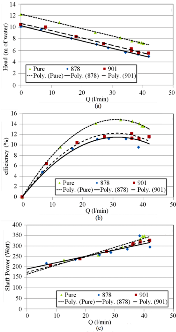
Figure 7. Experimental relation between (a) head, (b) efficiency, and (c) shaft power and flowrate for pure water and oil of two different densities (878 and 901 kg/m 3 ) with a concentration of 0.01 at 1535 rpm, respectively.
