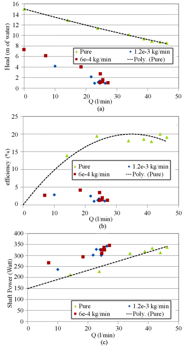
Figure 14. Experimental relation between (a) head, (b) efficiency, and (c) shaft power and flowrate for different air flowrate values at 1650 rpm and 3rd stage, respectively.
