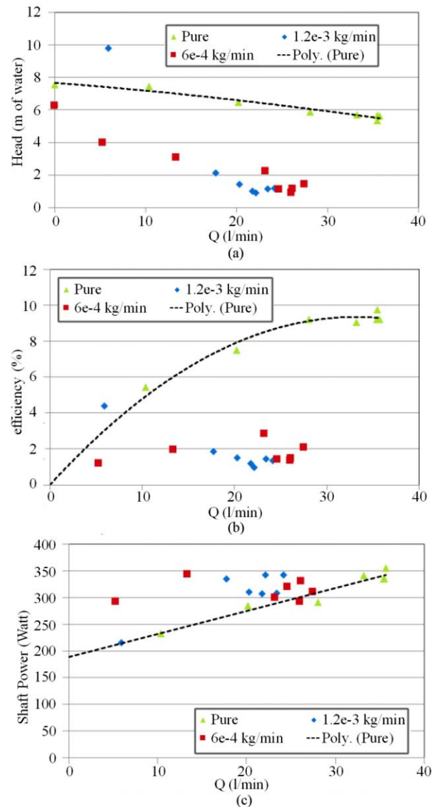
Figure 12. Experimental relation between (a) head, (b) efficiency, and (c) shaft power and flowrate for different air flowrate values at 1400 rpm and 3rd stage, respectively.
