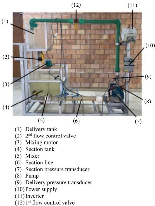
Figure 1. The test rig.
