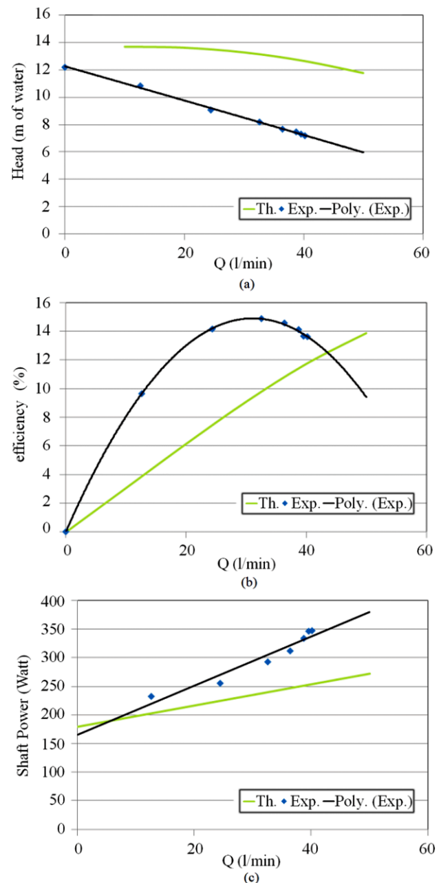
Figure 2. Comparison between analytical and experimental relation between (a) head, (b) efficiency, and (c) shaft power and flowrate for pure water at 1535 rpm, respectively.
