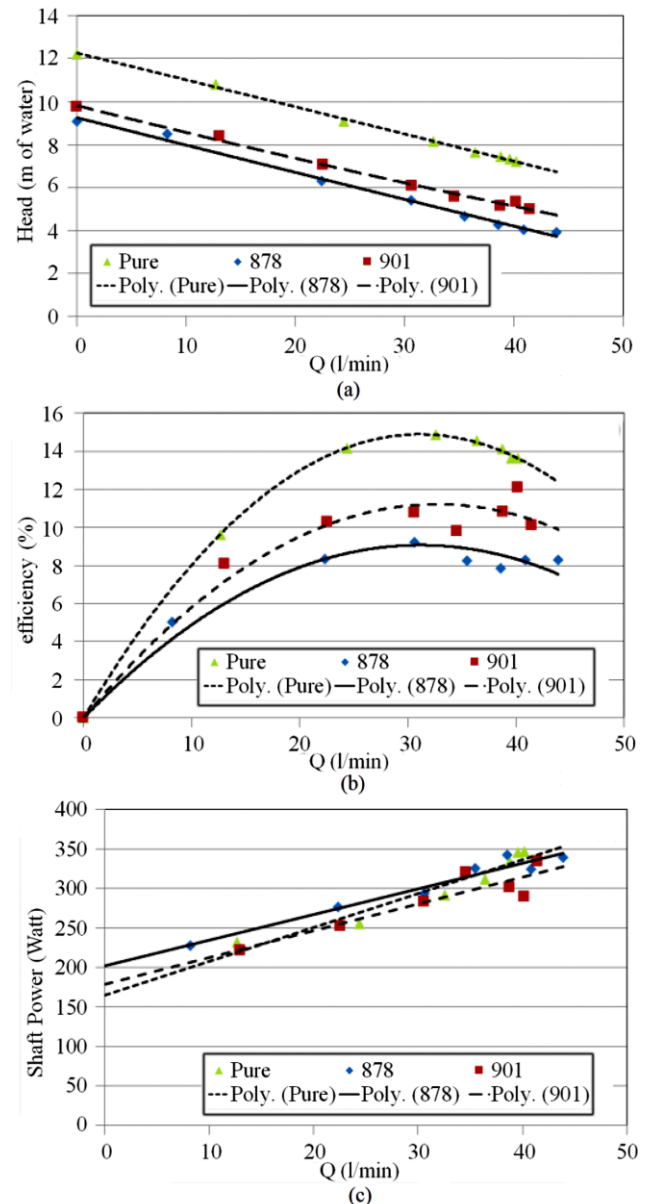
Figure 8. Experimental relation between (a) head, (b) efficiency, and (c) shaft power and flowrate for pure water and oil of two different densities (878 and 901 kg/m 3 ) with a concentration of 0.02 at 1535 rpm, respectively.
