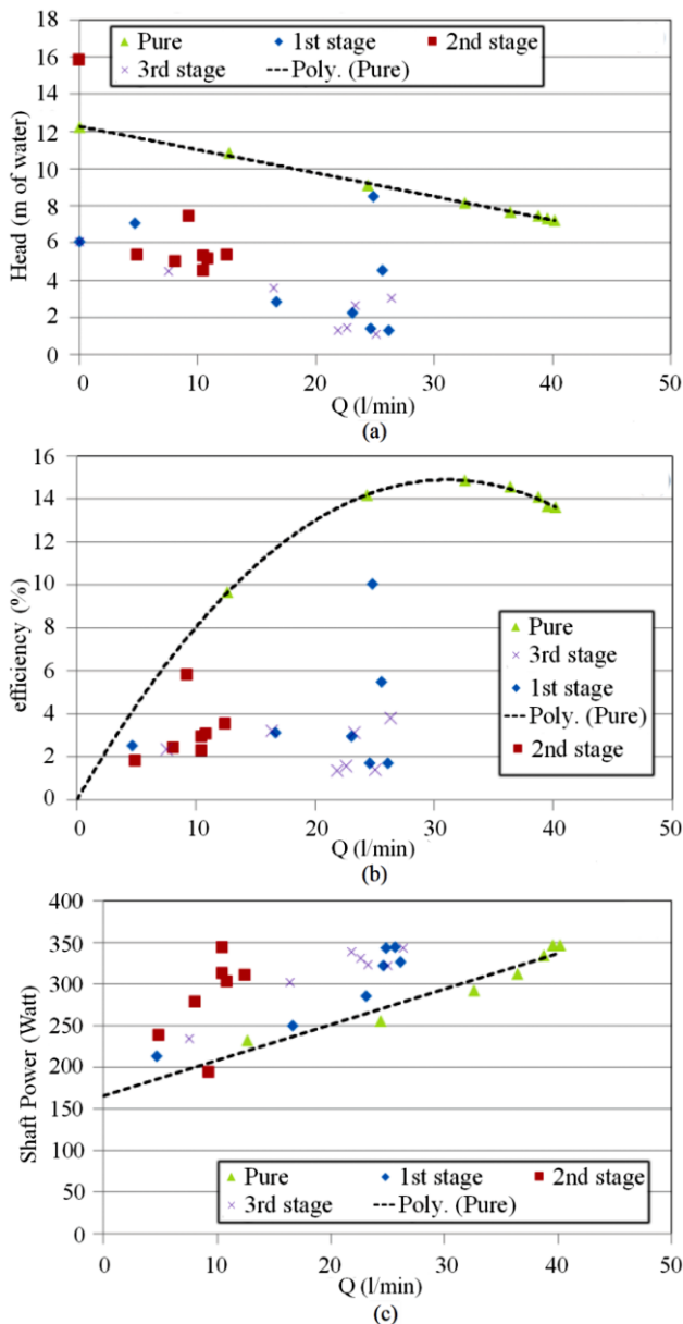
Figure 10. Experimental relation between (a) head, (b) efficiency, and (c) shaft power and flowrate for pure water and 1 lpm ( 1.2 \times 10^{-3} kg/min) air inserted at 1st, 2nd and 3rd stages at 1535 rpm, respectively.
