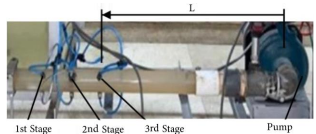
Figure 9. The transparent pipe and the three stages.
