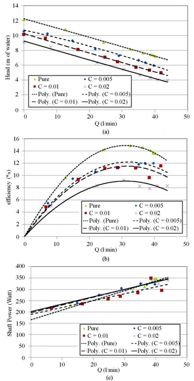
Figure 4. Experimental relation between (a) head, (b) efficiency, and (c) shaft Power and flowrate for pure water and oil of density of 878 kg/m³ with different concentrations at 1535 rpm, respectively.
