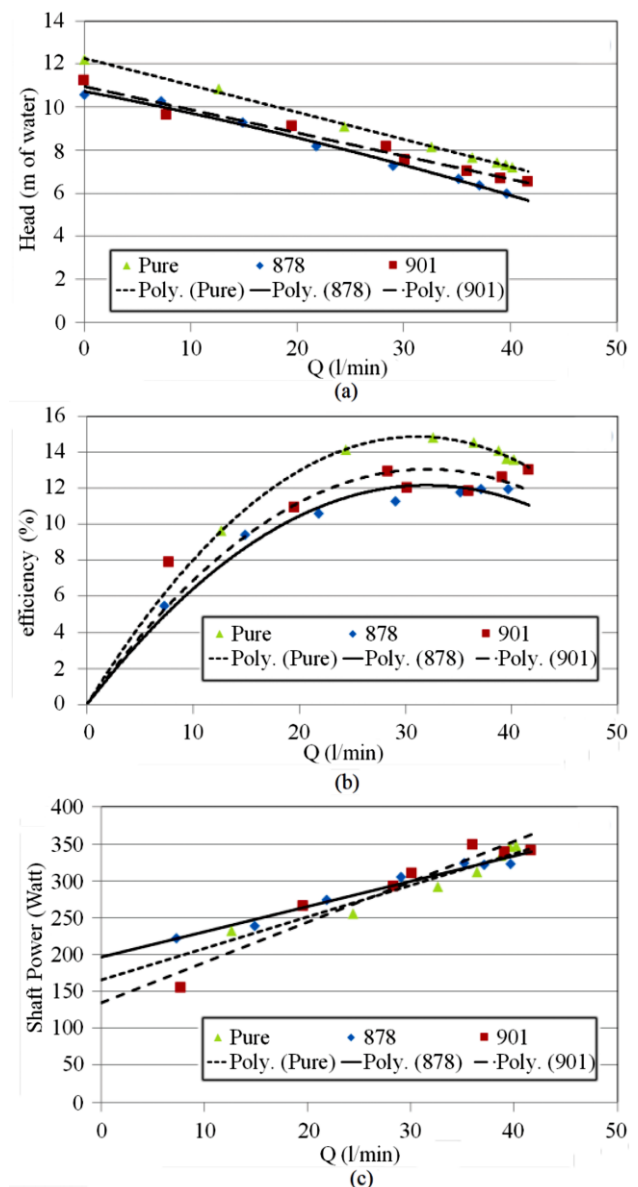
Figure 6. Experimental relation between (a) head, (b) efficiency, and (c) shaft power and flowrate for pure water and oil of two different densities ( 878 and 901 \text{ kg/m}^3 ) with a concentration of 0.005 at 1535 rpm, respectively.
