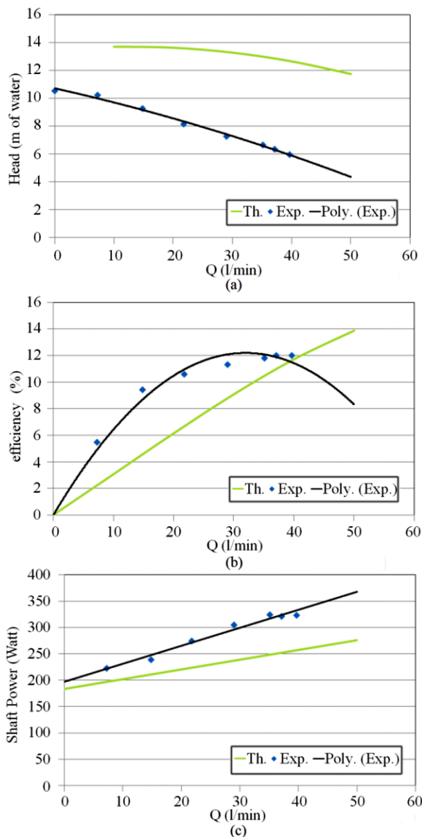
Figure 5. Comparison between analytical and experimental relation between (a) head, (b) efficiency, and (c) shaft power and flowrate for oil of density 878 \text{ kg/m}^3 with a concentration of 0.005 at 1535 rpm, respectively.
