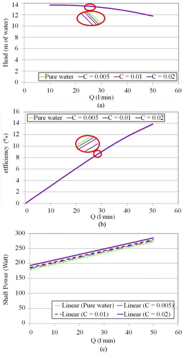
Figure 3. Analytical relation between (a) head, (b) efficiency, and (c) shaft power and flowrate for pure water and oil of density of 878 kg/m³ with different concentrations at 1535 rpm, respectively.
