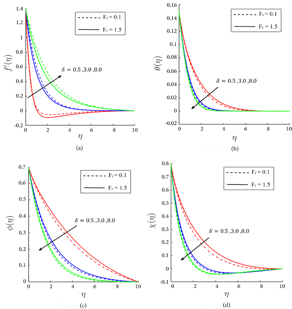
Figure 3. Distribution of f'(\eta) , \theta(\eta) , \phi(\eta) and \chi(\eta) for \delta and F_r .
