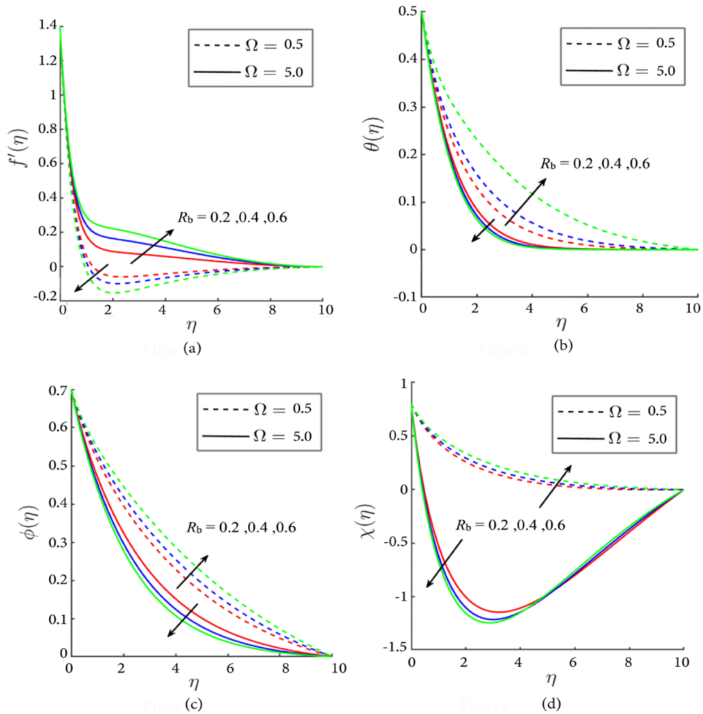
Figure 2. Distribution of f'(\eta) , \theta(\eta) , \phi(\eta) and \chi(\eta) for \Omega and R_b .
