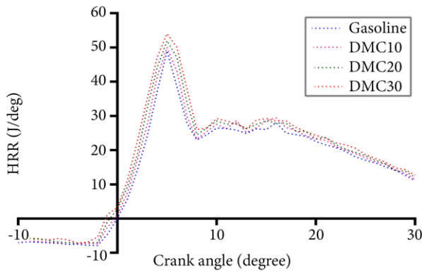
Figure 11. Heat release rate versus crank angle.
