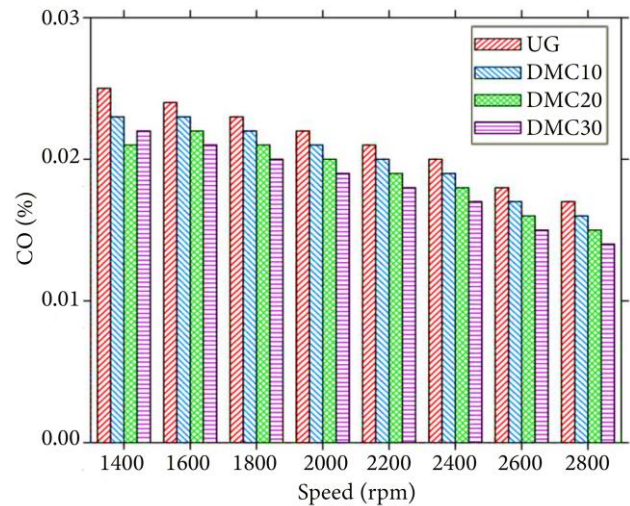
Figure 8. CO emission for different engine speeds.
