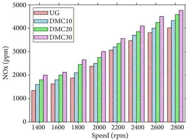
Figure 9. NO x emissions for different engine speeds.
