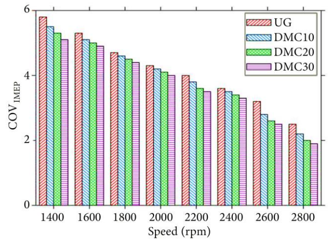
Figure 6. COV_{IMEP} for different engine speeds.
