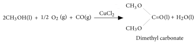
Figure 3. Synthesis of DMC.
