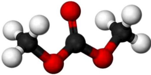
Figure 4. Molecular structure of DMC.
