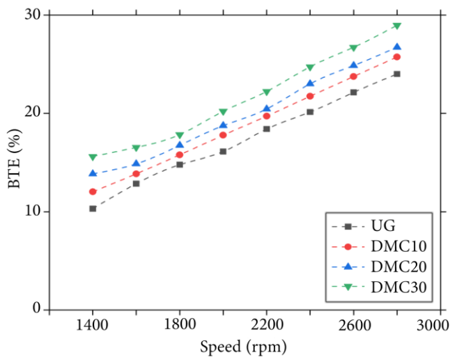
Figure 5. BTE for different engine speeds.
