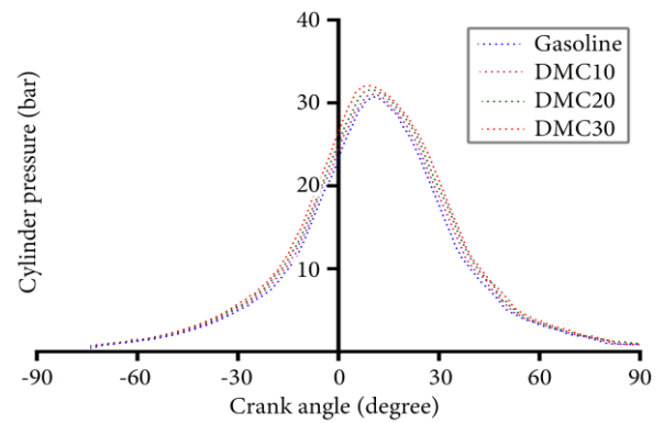
Figure 10. In-cylinder pressure versus crank angle.
