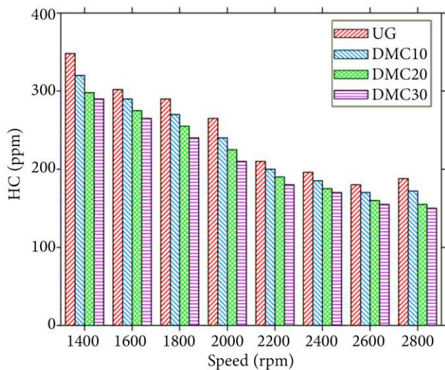
Figure 7. HC emission for different engine speeds.
