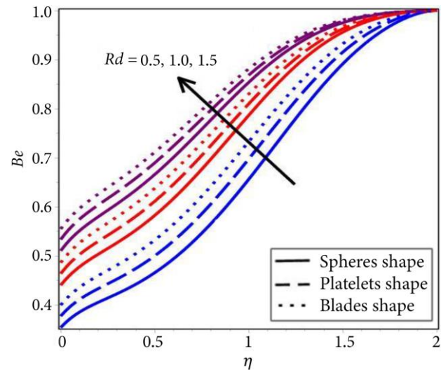
Figure 14. The behaviour of Be with specific values of Rd .
