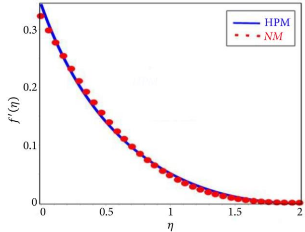
Figure 2. Comparison of the R-K method with the HPM for velocity profile.
