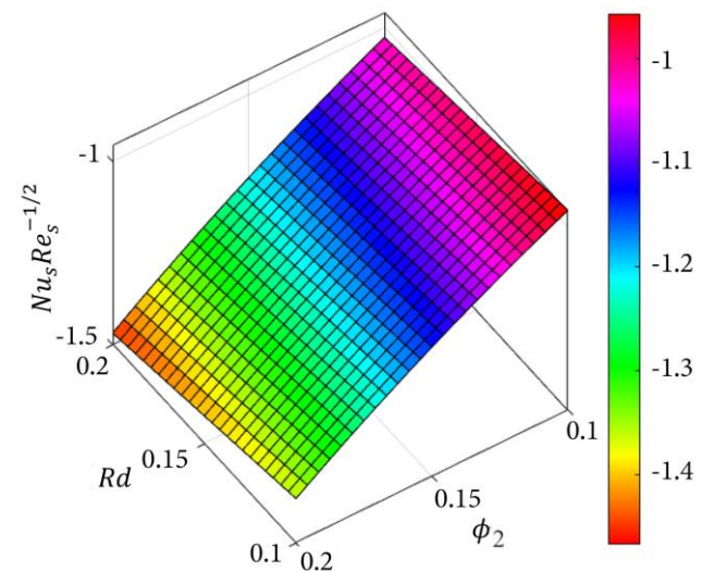
Figure 20. The variant of \phi_2 and Rd on Nu_s Re_s^{-1/2} .
