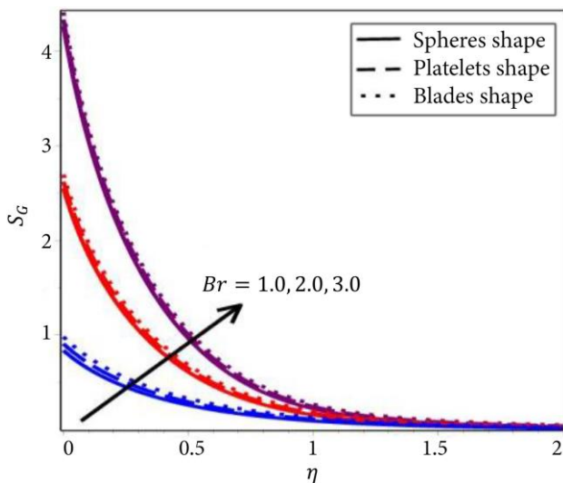
Figure 11. The behavior of S_G with specific values of Br .
