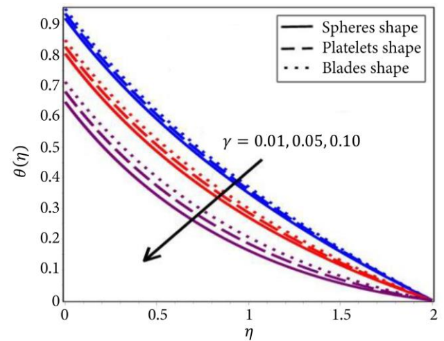
Figure 8. The behavior of \theta(\eta) with specific values of \gamma .
