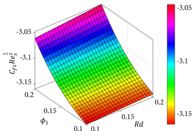
Figure 18. The variant of \phi_1 and Rd on C_{fs} Re_s^{1/2} .
