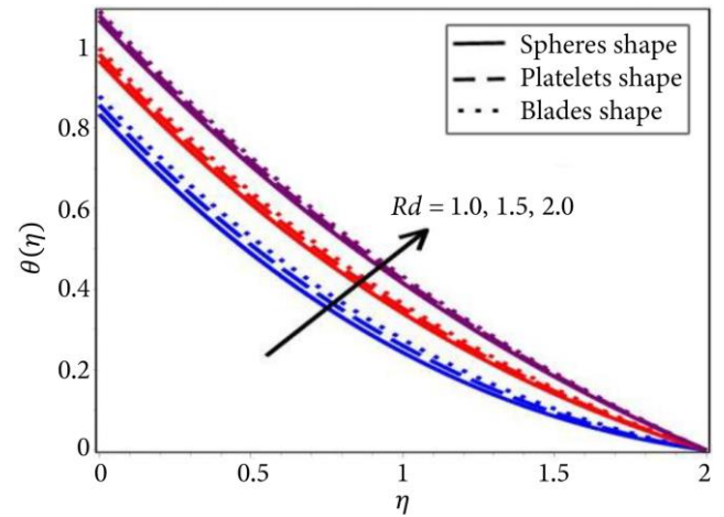
Figure 7. The behavior of \theta(\eta) with specific values of Rd .
