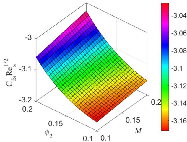
Figure 17. The variant of \phi_2 and M on C_{fs} Re_s^{1/2} .
