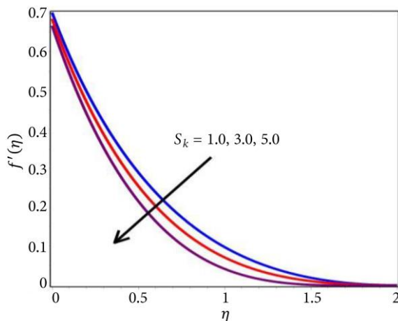
Figure 6. The behavior of f'(\eta) with specific values of S_k .
