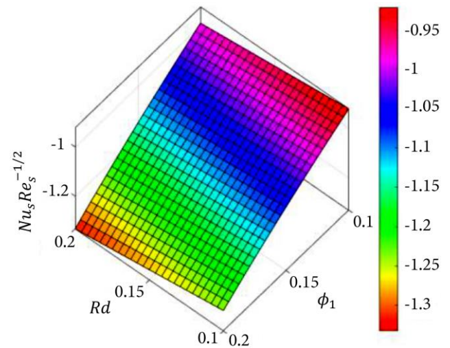
Figure 19. The variant of \phi_1 and Rd on Nu_s Re_s^{-1/2} .
