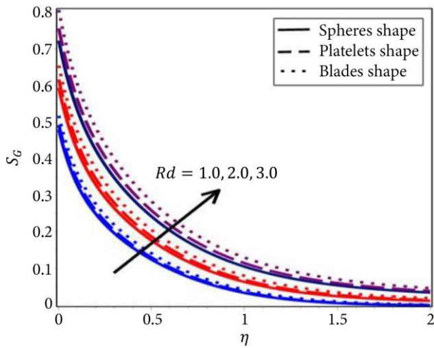
Figure 10. The behavior of S_G with specific values of Rd .
