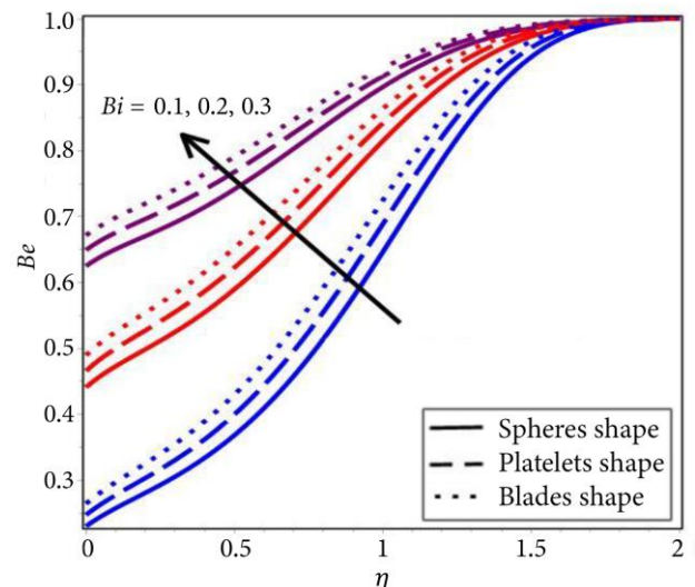
Figure 15. The behavior of Be with specific values of Bi .
