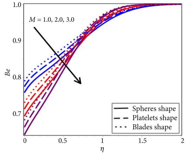
Figure 13. The behavior of Be with specific values of M .
