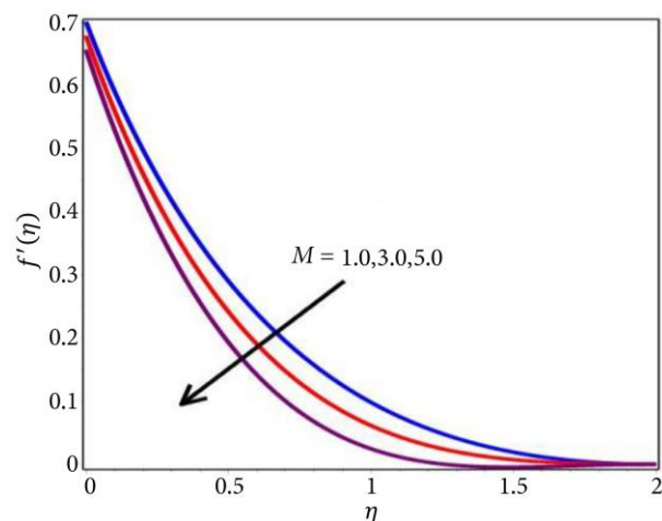
Figure 4. The behavior of f'(\eta) with different values of M .
