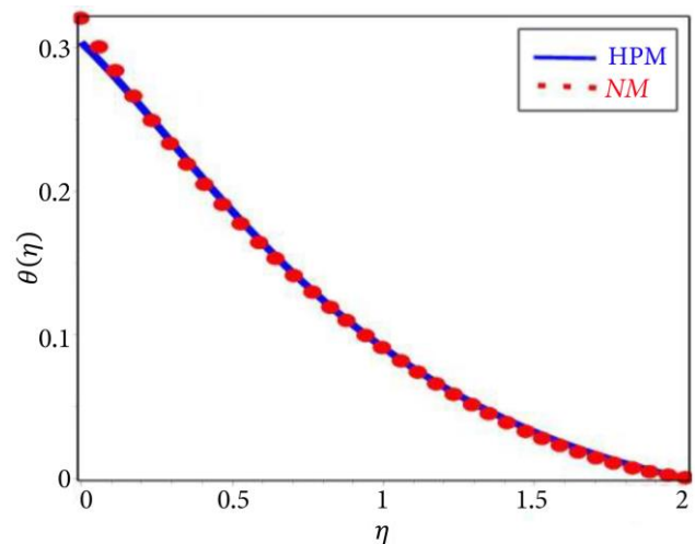
Figure 3. Comparisons of the R-K method with the HPM for temperature profile.
