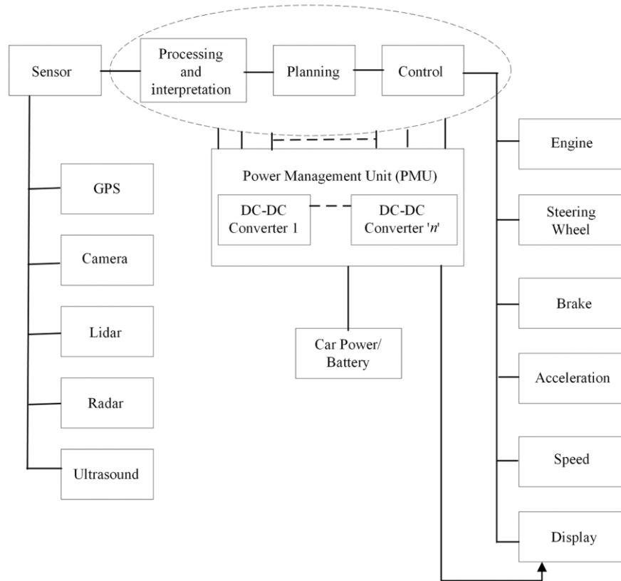
Figure 1. Block diagram of an autonomous vehicle with major electronic systems.
