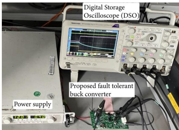
Figure 7. Experimental set-up of proposed system.
