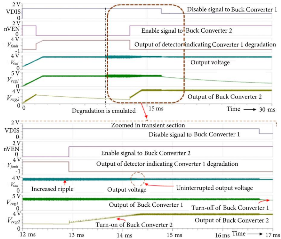
Figure 5. Simulation result of the proposed method. Here, V_{reg1} and V_{reg2} are the output voltages from Buck Converter 1 and Buck Converter 2 respectively. V_{fault} is the fault-indicating signal. nVEN and VDIS are enable signal given to Buck Converter 2 and disable signal given to Buck Converter 1 respectively.
