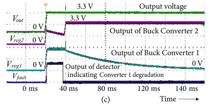
Figure 8 (a) Output of the proposed system during Turn-ON and upon healthy operation; (b) experimental results of proposed fault-tolerant buck converter upon fault occurrence during operation; and (c) output of the proposed system upon Turn-ON while regulator1 is degraded.
