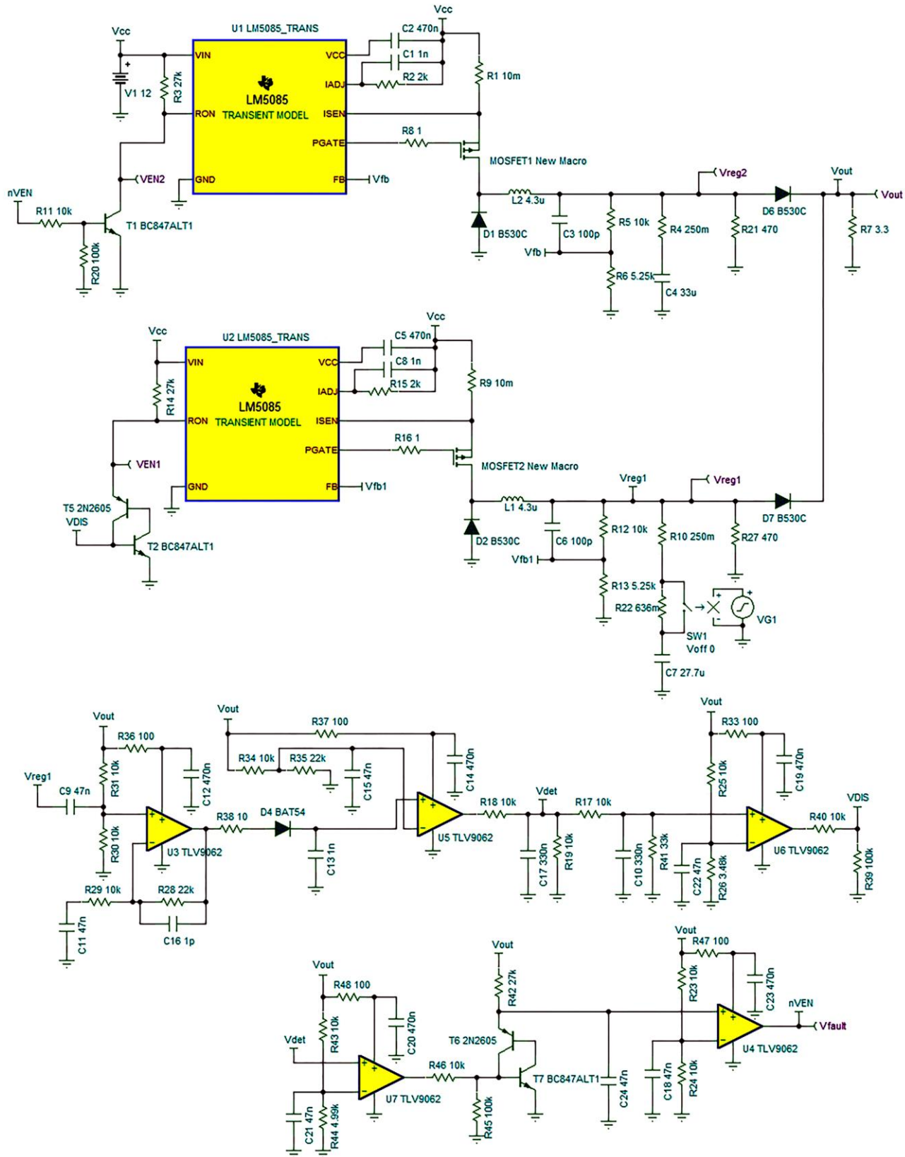
Figure 4. Schematic representation of proposed fault-tolerant scheme.
