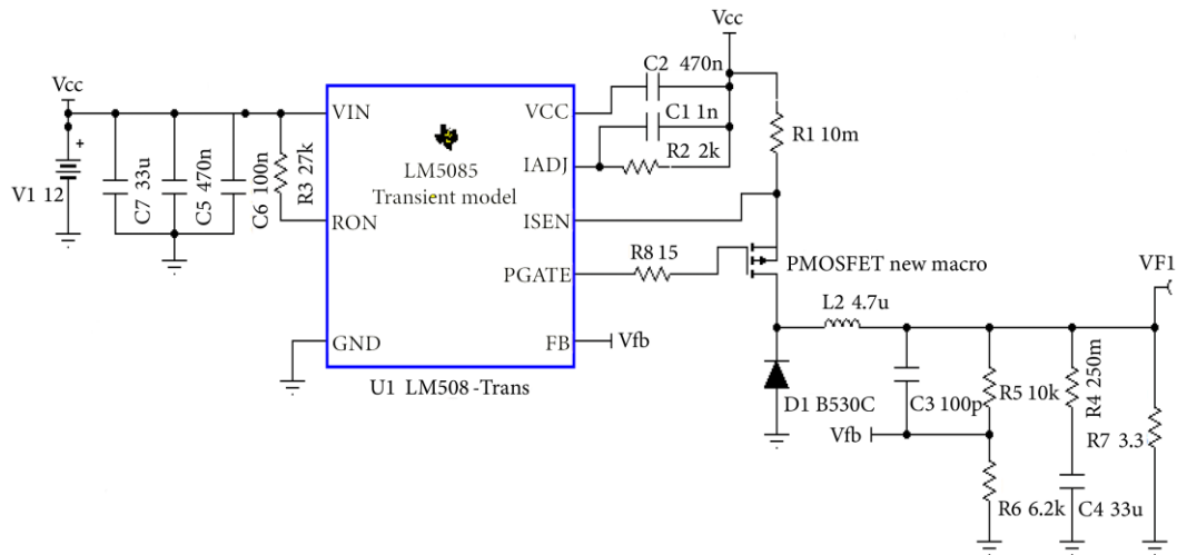
Figure 3. Schematic of the voltage regulator designed.
