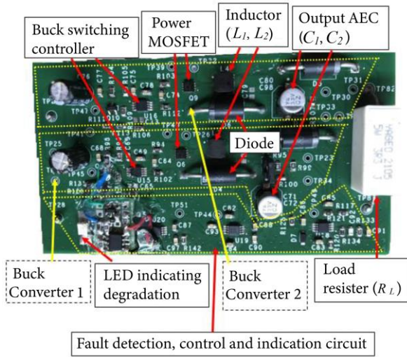
Figure 6. Prototype of proposed solution.
