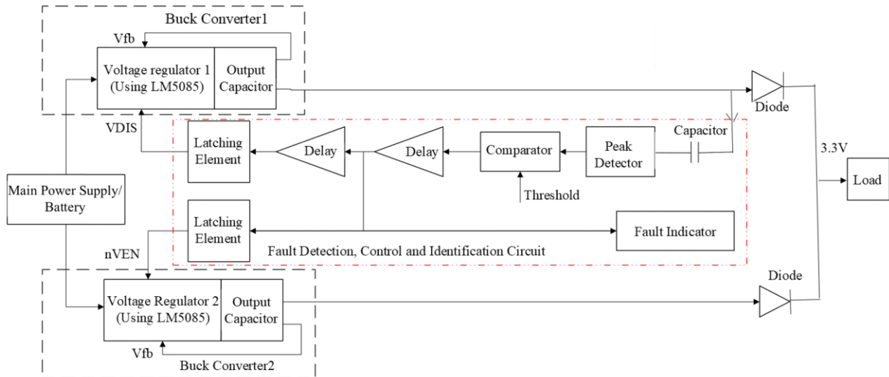
Figure 2. Block diagram of proposed solution.
