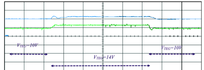
(a) Output voltage ( V_{TEG} , blue waveform, 2.5 V/Div ) and current ( I_{TEG} , Green waveform, 3.75 A/Div ) of TEG source. Time-division is 5 ms.
