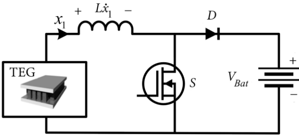
Figure 4. Application of the TEG as an input power source of a boost DC-DC converter.
