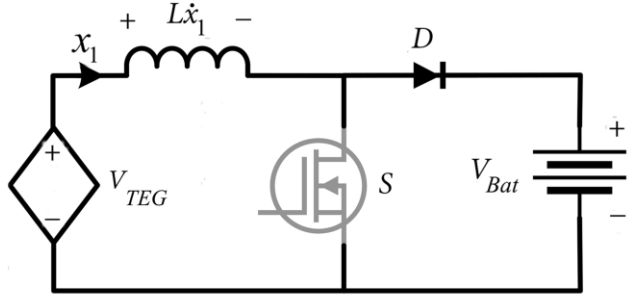
(b) The power switch (S) is off
