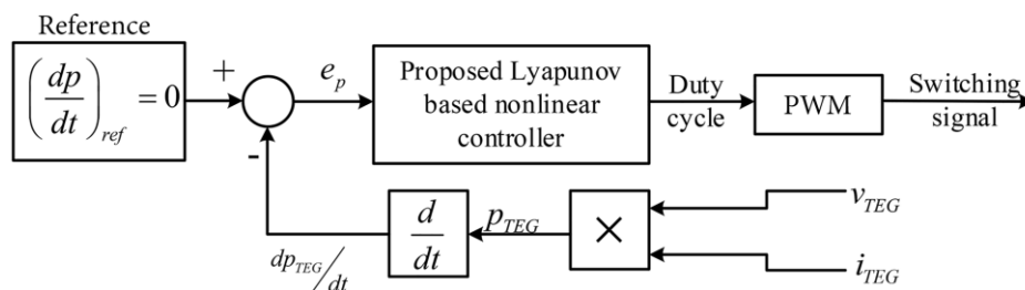
Figure 7. The block diagram of the proposed Lyapunov-based nonlinear controller.
