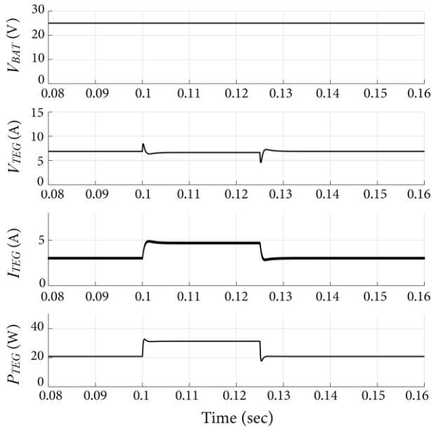
Figure 13. Simulation of the controller during periodic changes of TEG internal resistance.
