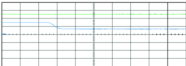
(b) Output voltage ( V_{TEG} , blue waveform, 10 V/Div.) of TEG source and load voltage ( V_{BAT} , Green waveform, 10 V/Div.). Time-division is 5 ms.
