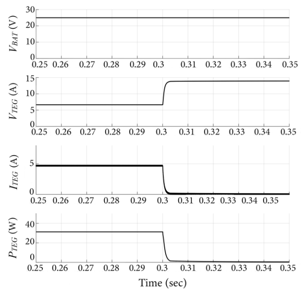
Figure 11. Shut-down response of the controller (simulation).
