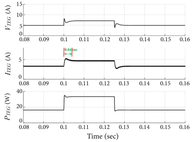
(a) Response of the developed controller
