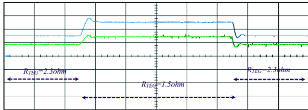
(b) Output power ( P_{TEG} , blue waveform, 10 W/Div ) and current ( I_{TEG} , Green waveform, 3.75 A/Div ) of TEG source. Time-division is 5 ms.
