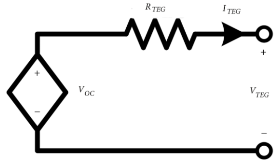
Figure 1. Equivalent electrical model of TEG.
