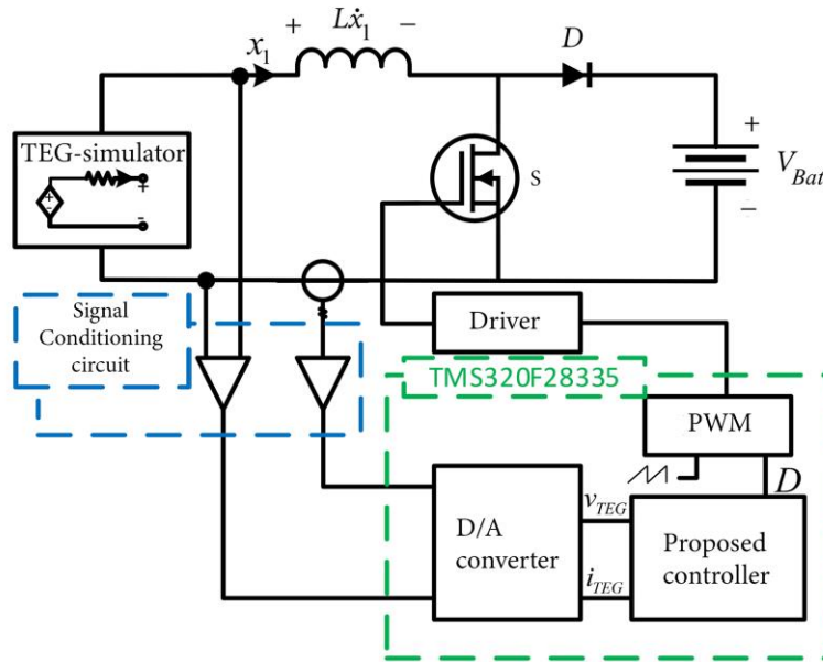
(b) Block diagram of the experimental setup
