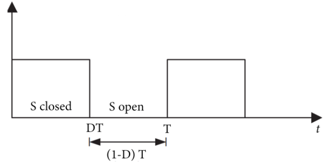
Figure A.1. Switching signal of DC-DC converters.
