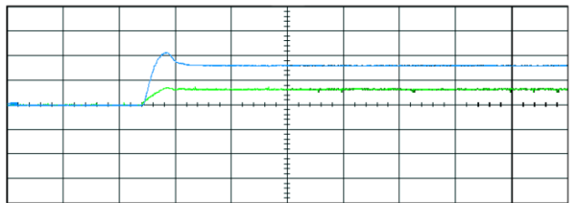
(c) Output power ( P_{TEG} , blue waveform, 25 W/Div.) and current ( I_{TEG} , Green waveform, 7.2 A/Div.) of the TEG source. Time-division is 5 ms.
