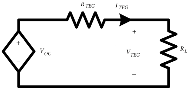
Figure 3. The output power of TEG depends on the external load.
