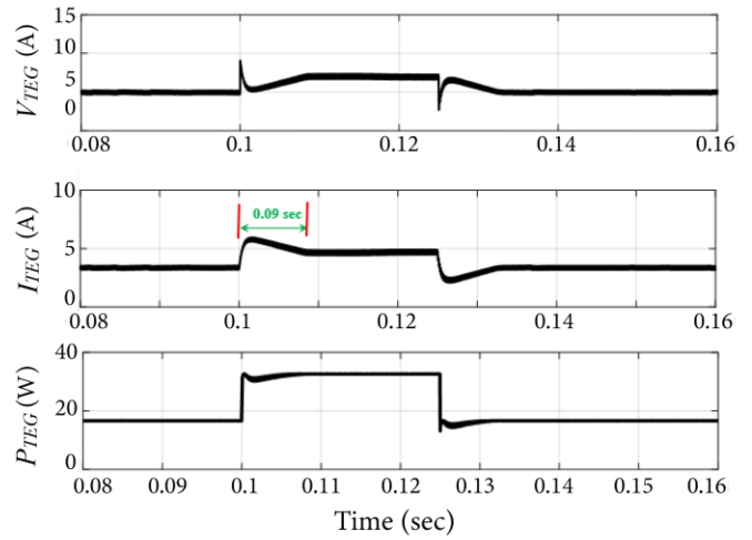
(b) Response of the two-loop P&O-based MPPT controller
