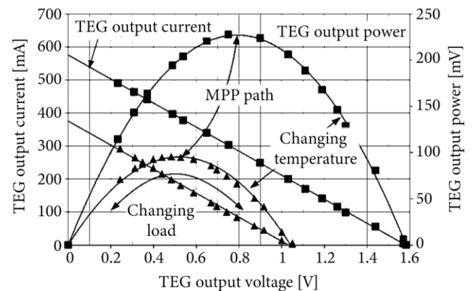
Figure 2. Current-voltage and power-voltage characteristics of a typical TEG for different temperatures [30].
