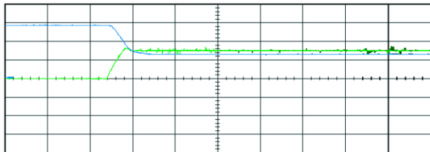
(a) Output voltage ( V_{TEG} , blue waveform, 5 V/Div.) and current ( I_{TEG} , Green waveform, 3.7 A/Div.) of TEG source. Time-division is 5 ms.
