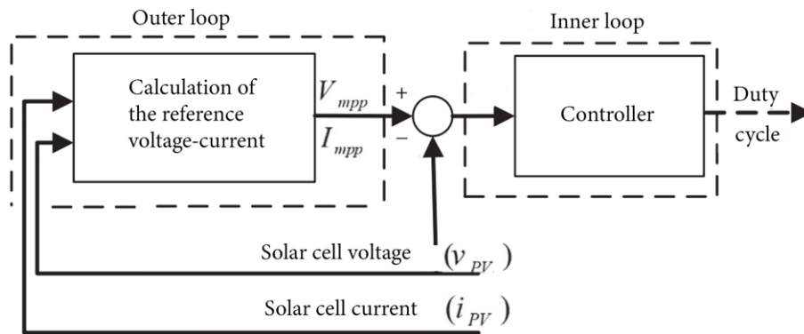
Figure 6. Two-loop controller for MPPT of TEG sources.
