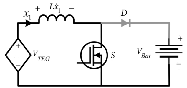
(a) The power switch (S) is on
