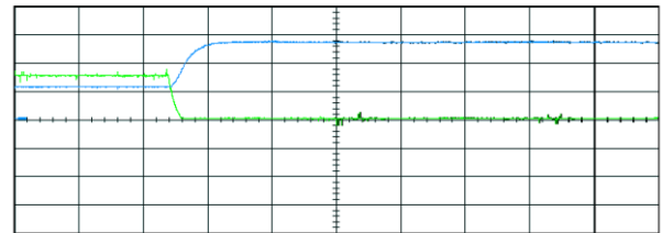
Figure 12. Experimental shut-down response of the converter. Output voltage ( V_{TEG} , blue waveform, 5V/Div.) and current ( I_{TEG} , Green waveform, 3.7A/Div.) of the TEG source are shown. The time division is 5 ms.
