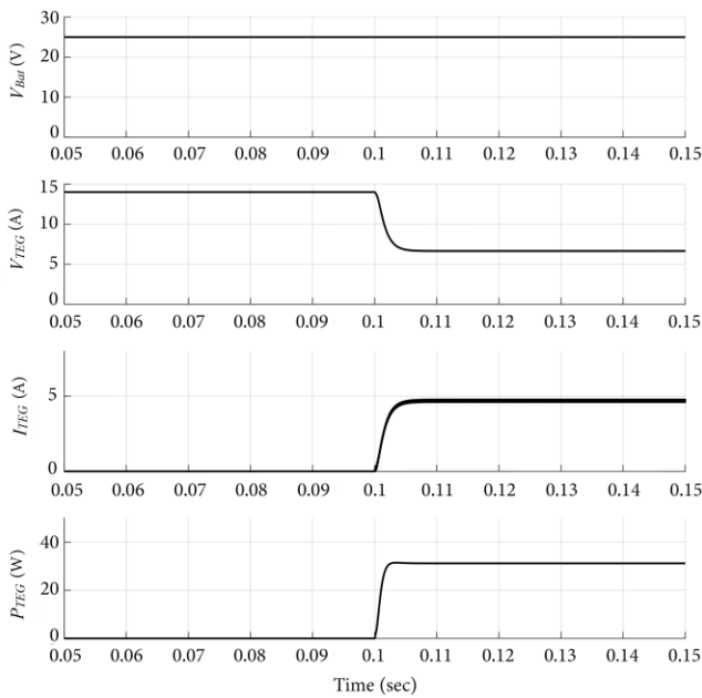
Figure 9. Dynamic response of the proposed controller during start-up (simulation).
