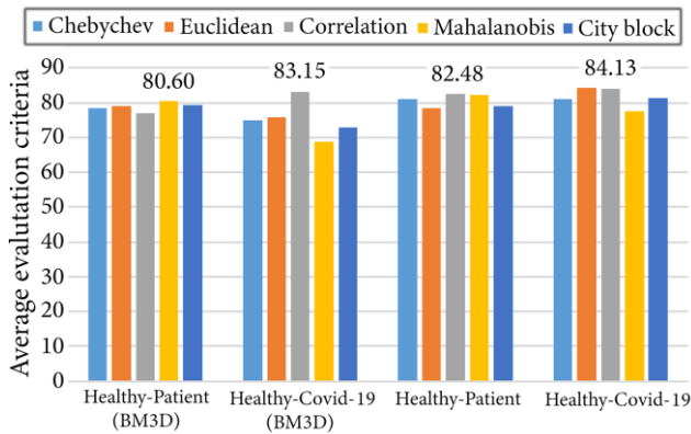
Figure 12. Comparison of distances in filtered and unfiltered images in different classes with FBSWT.
