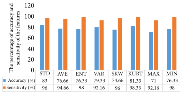
Figure 9. Evaluation of the performance of feature selection within the ML framework.
