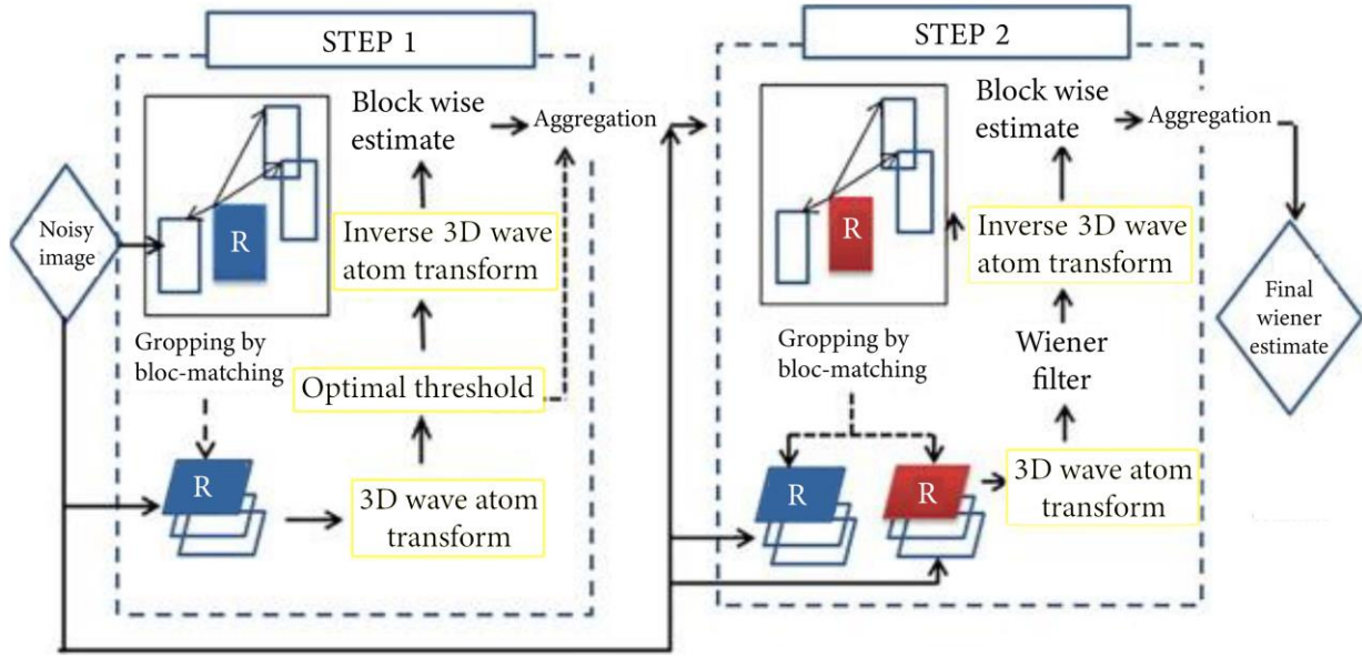
Figure 4. Scheme of the BM3D algorithm [26].
