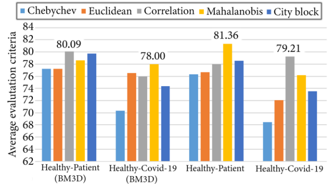
Figure 11. Comparison of distances in filtered and unfiltered images of different classes in WT
