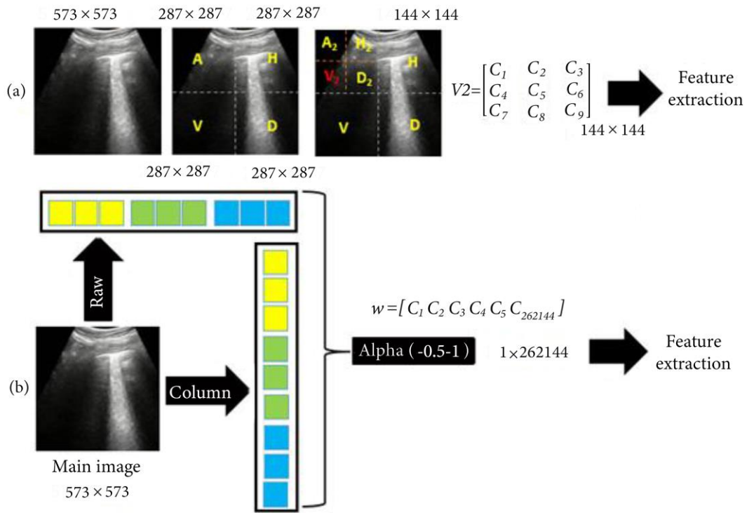
Figure 7. Extracting the primary feature: (a) The WT and (b) the FBSWT.
