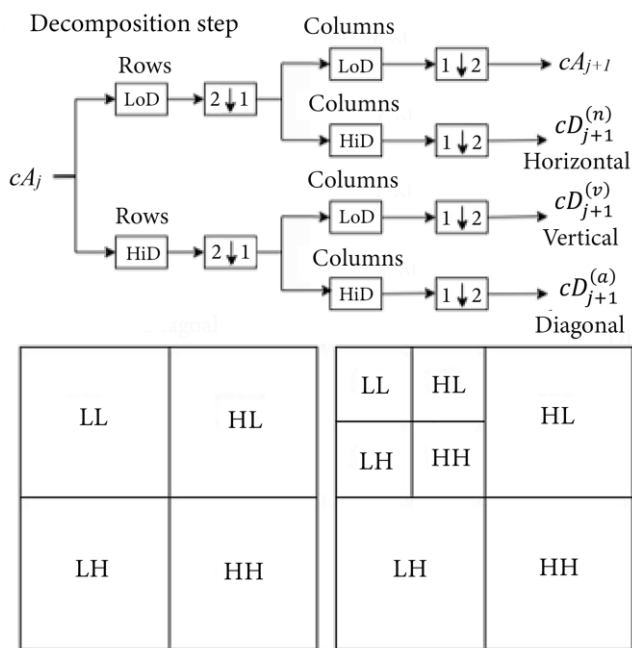
Figure 6. Decomposition of the image into two levels of decomposition and extraction of primary features [28].
