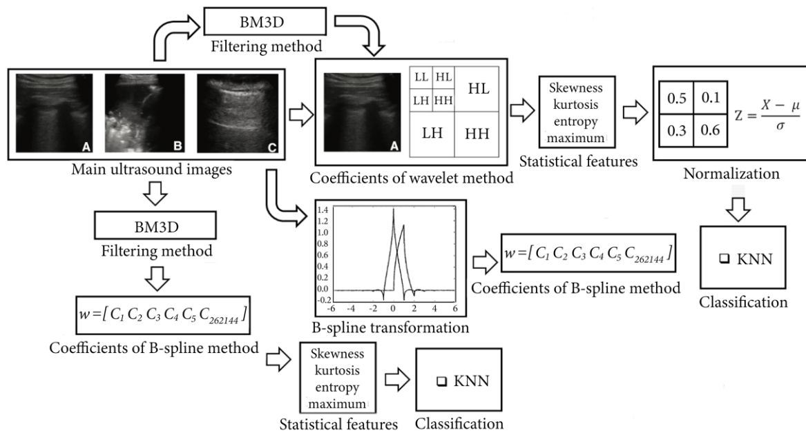
Figure 2. Outline of the proposed method for classifying healthy people from patients.
