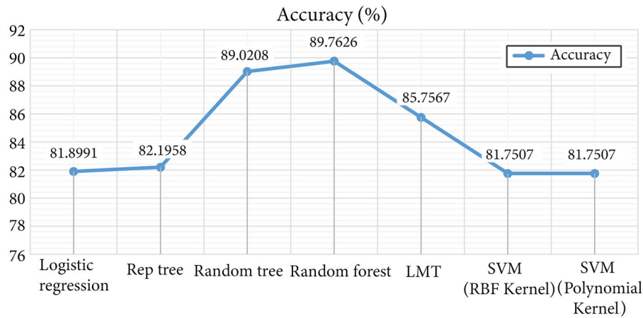
Figure 3. The accuracies of classifiers.
