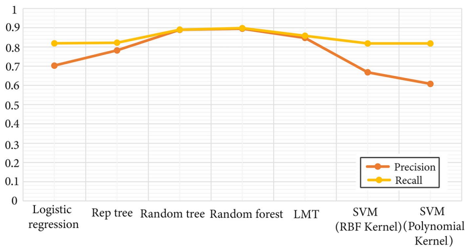
Figure 4. Precision and Recall metrics of classifiers.
