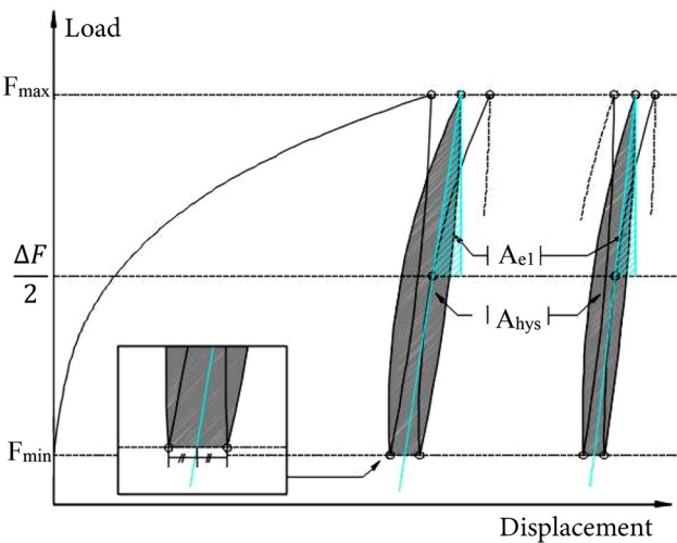
Figure 25. Definition of the cyclic damping ratio.
