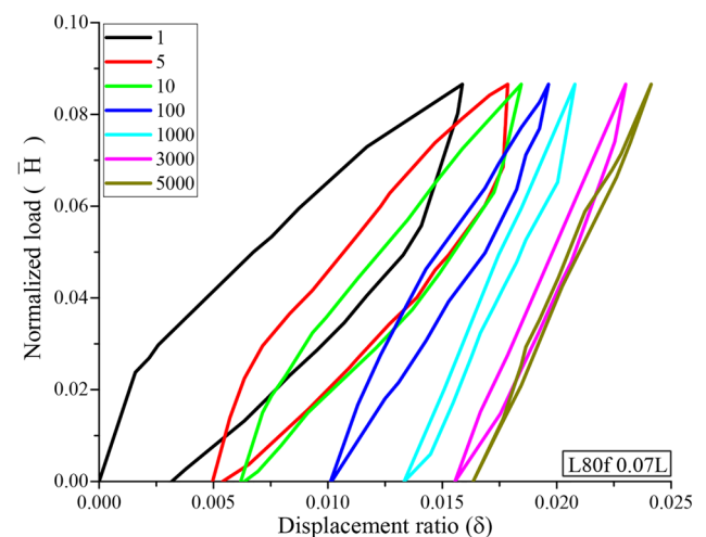
Figure 20. Normalized lateral load and horizontal displacement relationship at various cycles for L80f0.07L.
