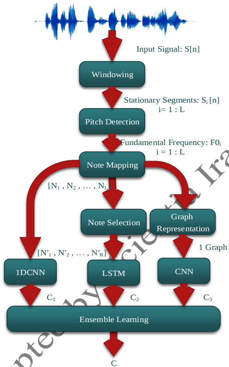
Fig. 1 Proposed method for dastgah recognition
