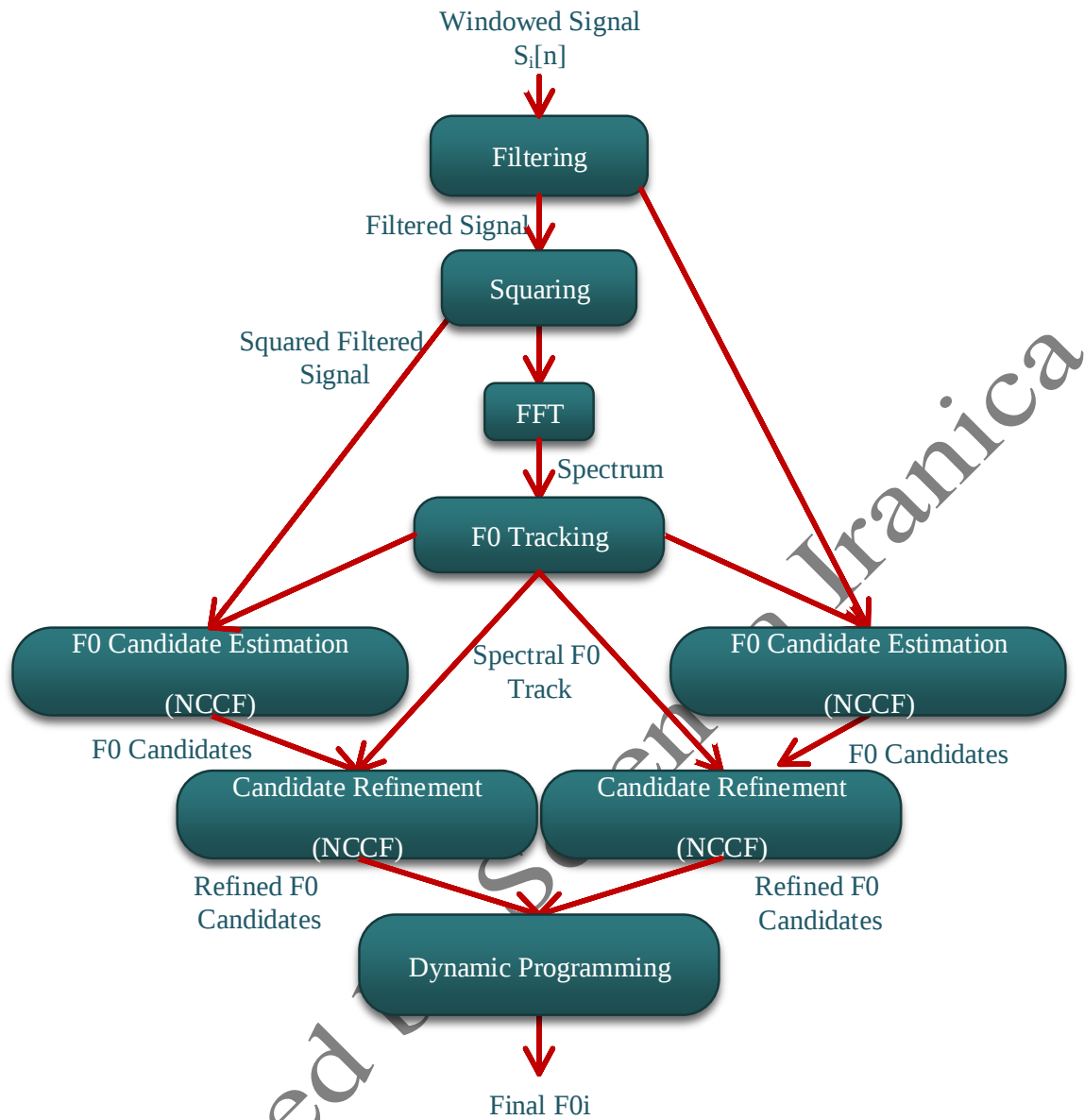
Fig. 2 YAAPT algorithm for pitch detection [48]
