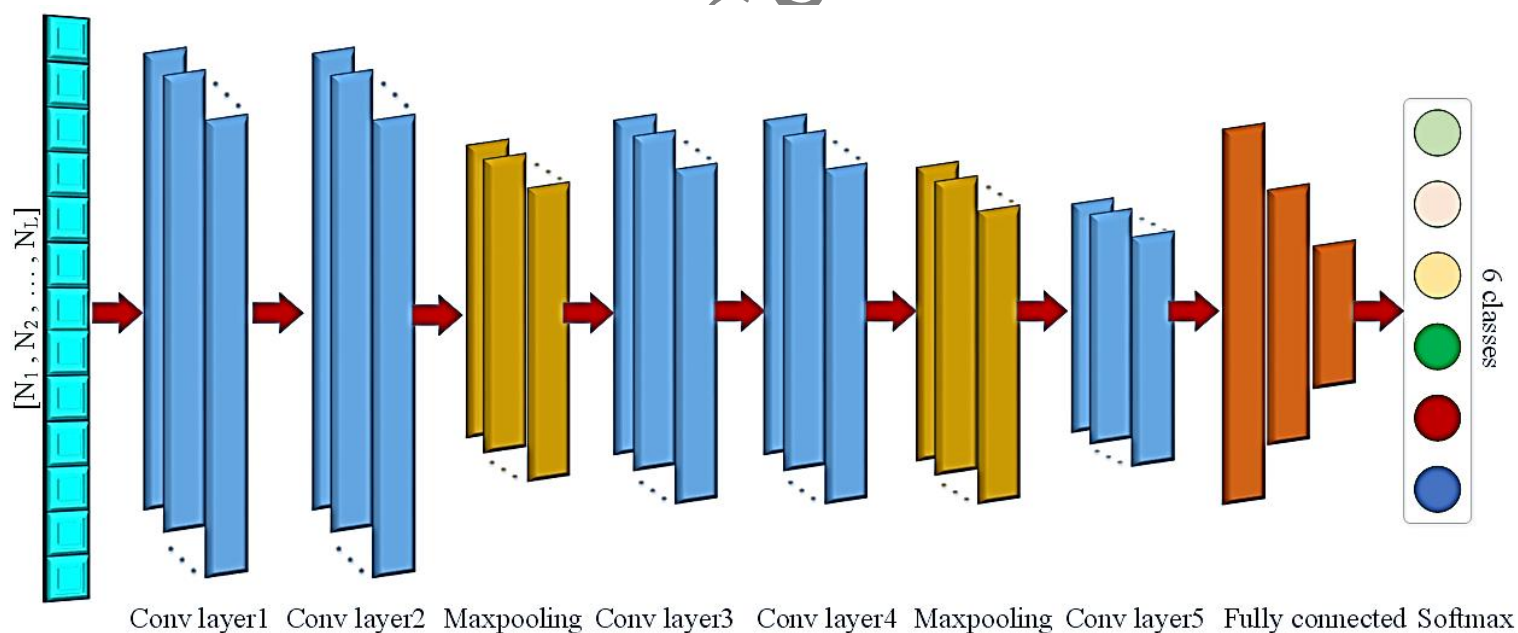
Fig. 3 1DCNN architecture for dastgah recognition
