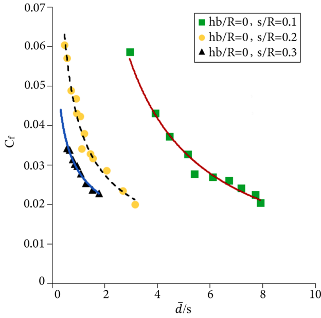
Figure 9. Fluid friction coefficient variation versus relative depth ratio ( d/s ) for h_b/R = 0 and s/R = 0.1, 0.2, 0.3 (slope = 20%).
