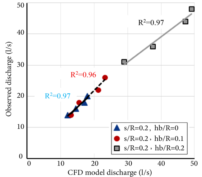
Figure 5. Physical and CFD models estimated discharge (l/s) for s/R = 0.2 .
