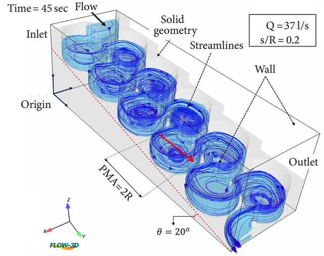
Figure 3. Three-dimensional solid geometry of MMCF and boundary condition used in CFD model.
