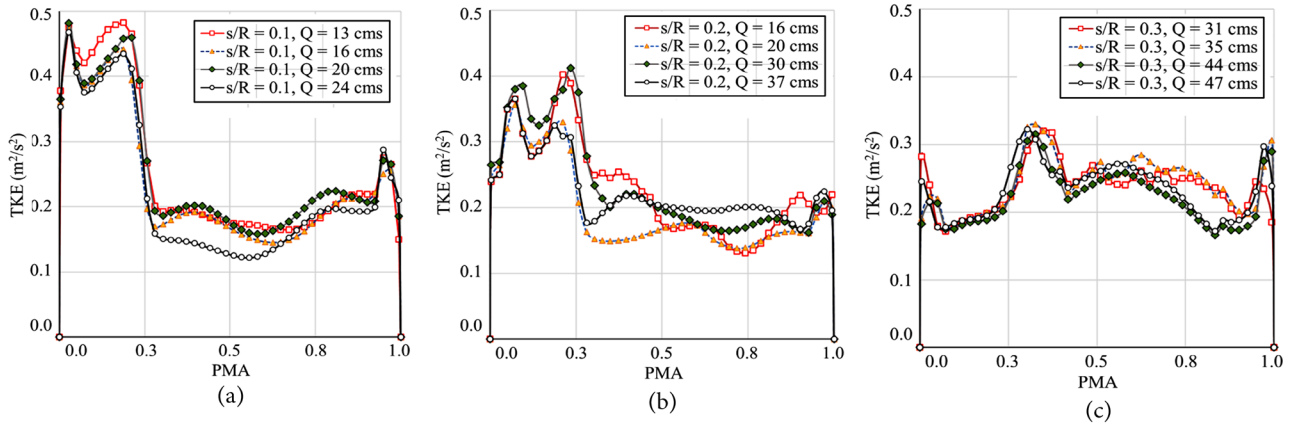
Figure 13. TKE variation through PMA for h_b/R = 0 (a) s/R = 0.1 , (b) s/R = 0.2 , and (c) s/R = 0.3 .
