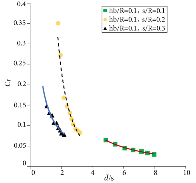
Figure 10. Fluid friction coefficient variation versus relative depth ratio ( d/s ) for h_b/R = 0.1 and s/R = 0.1, 0.2, 0.3 (slope = 20%).
