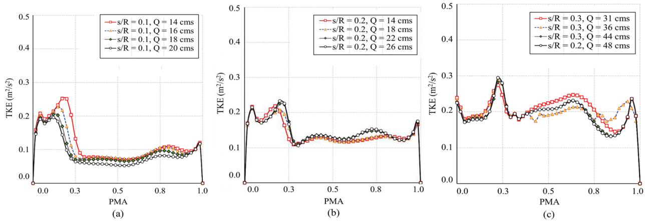
Figure 14. TKE variation through PMA for h_b/R = 0.1 (a) s/R = 0.1 , (b) s/R = 0.2 , and (c) s/R = 0.3 .
