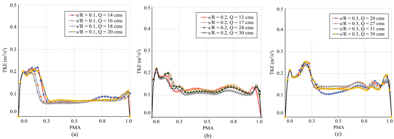
Figure 15. TKE variation through PMA for h_b/R = 0.2 (a) s/R = 0.1 , (b) s/R = 0.2 , and (c) s/R = 0.3 .
