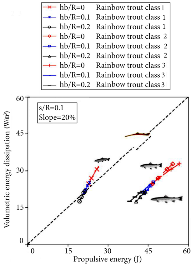
Figure 16. Potential volumetric energy ( W/m^3 ) in MMCF pools vs. propulsive energy (J) of three rainbow trout hypothetical classes ( s/R = 0.1 ).
