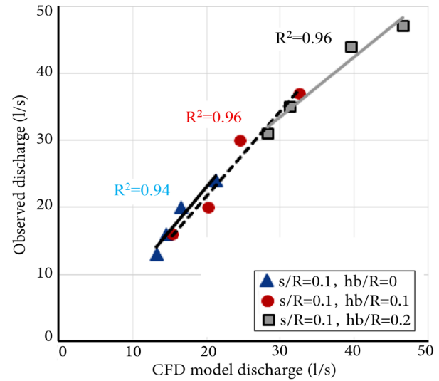
Figure 4. Physical and CFD models estimated discharge (l/s) for s/R = 0.1 .
