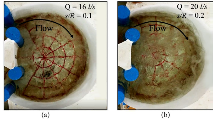
Figure 12. Qualitative assessment of flow in measuring pool No. 8 for (a) s/R = 0.1 and (b) s/R = 0.2 for d/s = 2.54 .
