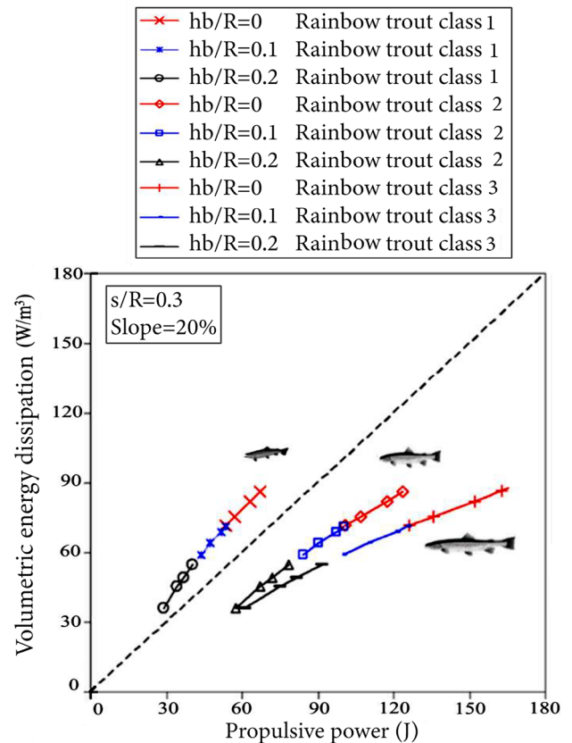
Figure 18. Potential flow volumetric energy ( W/m^3 ) in MMCF pools vs. propulsive energy (J) of three rainbow trout hypothetical classes ( s/R = 0.3 ).
