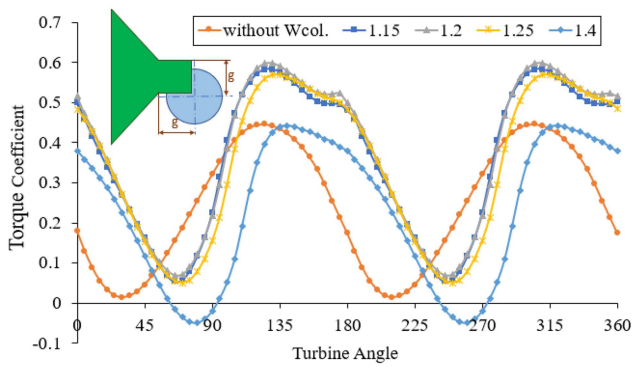
Figure 13. The effect of different ( g/R ) ratio on the torque-coefficient relative to the turbine-angle.
