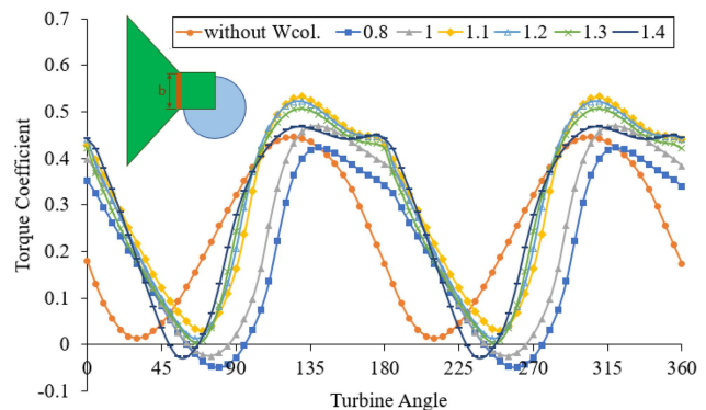
Figure 9. The effect of different ( b/R ) ratio on the coefficient of torque relative to the rotation angle of the turbine.
