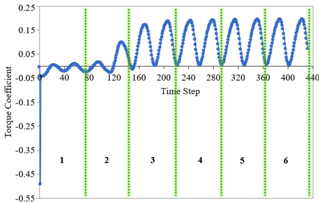
Figure 5. Stability study of the time step.
