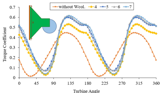
Figure 11. The effect of different ( a/R ) ratio on the torque-coefficient relative to the rotation angle.
