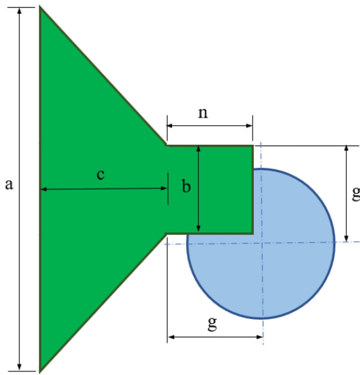
Figure 3. Geometric dimensions of wind collector.
