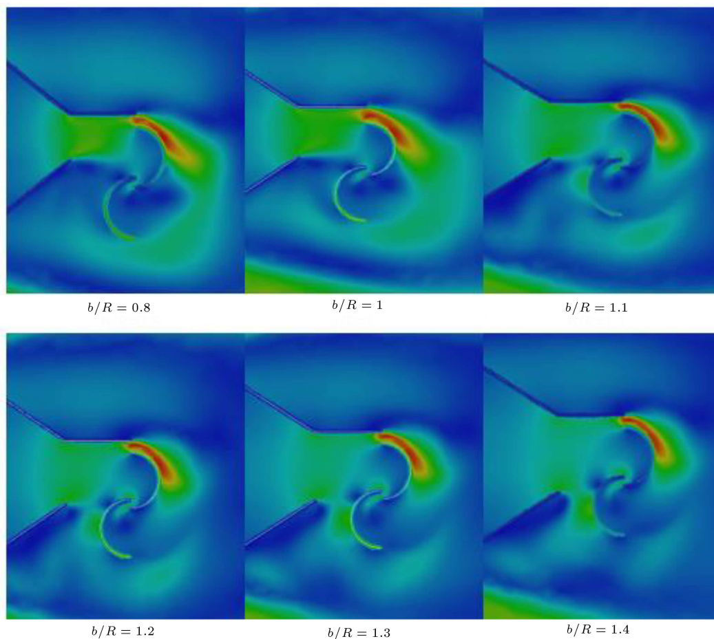
Figure 10. Velocity contours of various b/R ratios.
