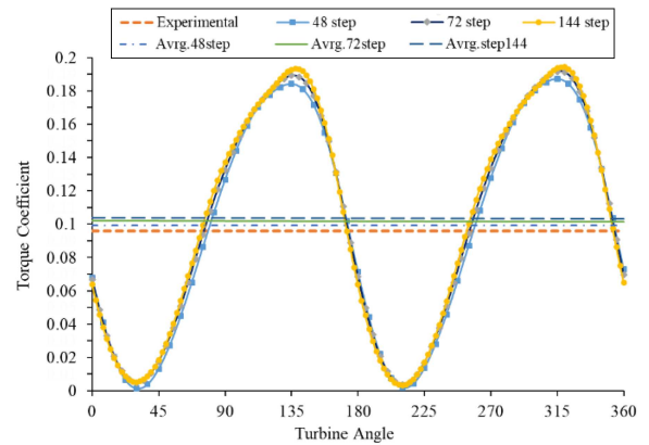
Figure 6. Time independence study of the time step.
