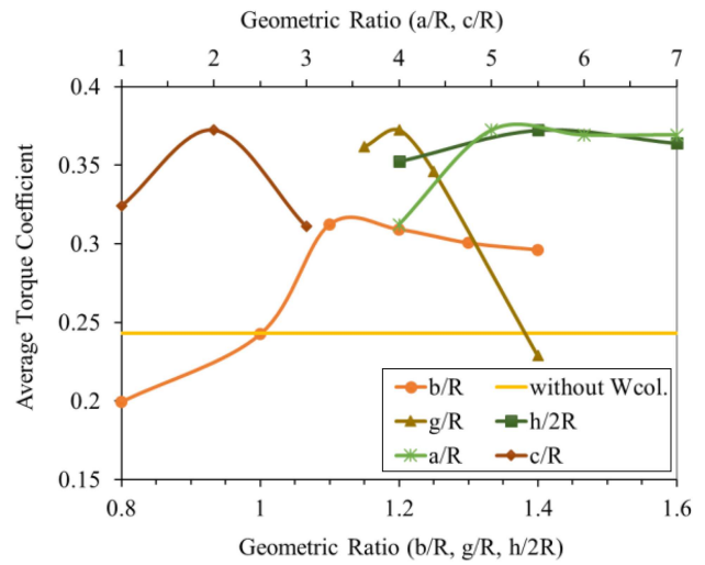
Figure 14. The effects of geometric wind collector parameter ratios on torque coefficient.
