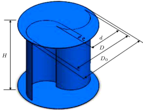
Figure 2. Dimensions of the SWT.
