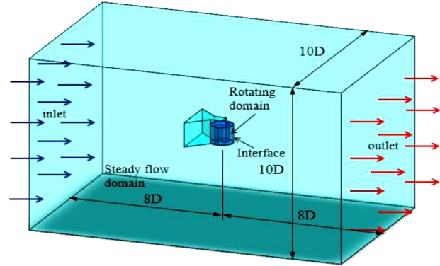
Figure 4. Computational domains and boundaries.
