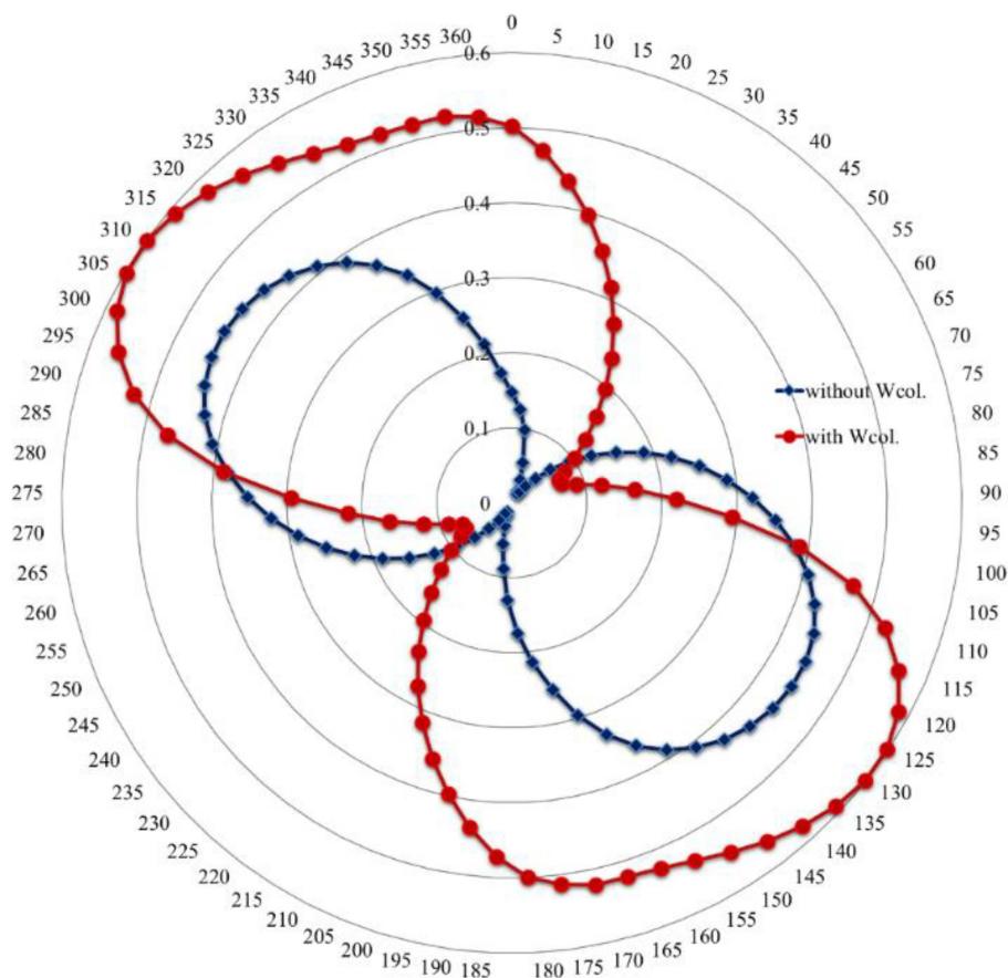
Figure 16. The change of the torque-coefficient at the maximum power-coefficient.
