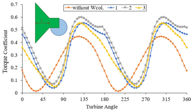
Figure 12. The effect of different ( c/R ) ratio on the torque-coefficient relative to the turbine-angle.
