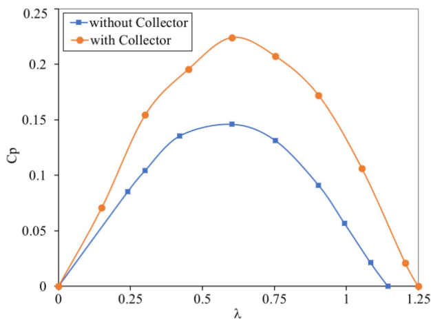
Figure 15. Change of the power-coefficient.
