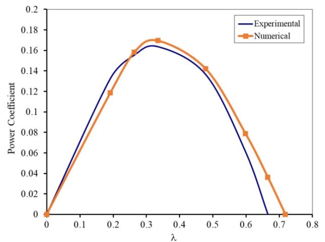
Figure 7. Verification of the numerical solution method.
