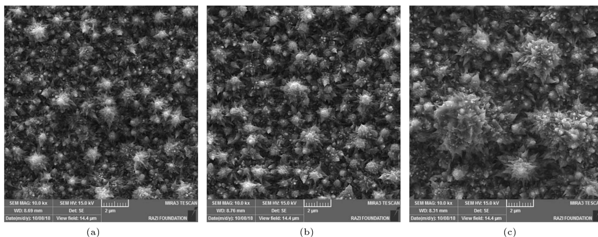
Figure 1. FESEM images of micro-nano hierarchically structured nickel coatings electrodeposited at current densities of: (a) 20 , (b) 40 , and (c) 60 mA/cm 2 .
