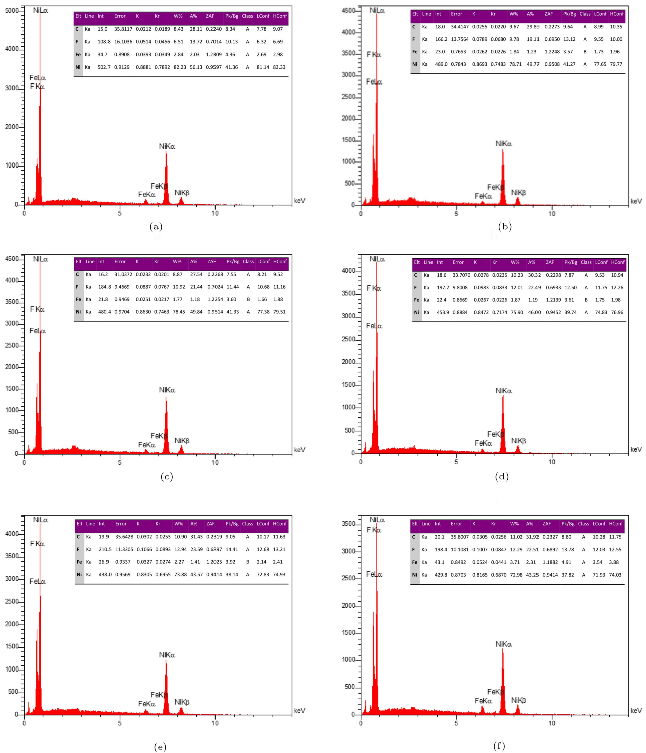
Figure 4. EDS spectra of Ni-PTFE coatings fabricated at different PTFE concentrations in electrodeposition bath: (a) 5, (b) 10, (c) 15, (d) 20, (e) 30, and (f) 40 g/L.
