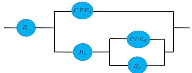
Figure 11. The equivalent circuits used to fit the EIS data.
