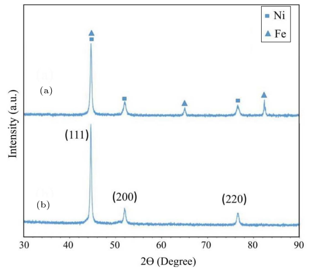
Figure 7. XRD spectra of: (a) Ni coating and (b) Ni-PTFE composite coating deposited at PTFE concentration of 15 g/L in electrodeposition bath.
