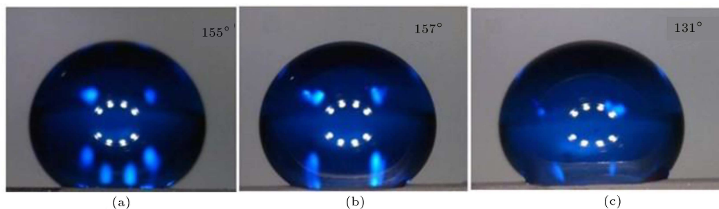
Figure 2. Contact angle of different hierarchically structured nickel coatings electrodeposited at current densities of: (a) 20, (b) 40, and (c) 60 mA/cm 2 .
