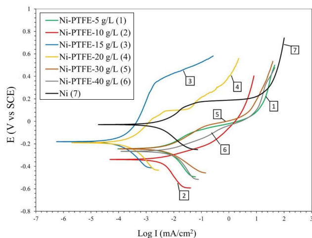
Figure 9. Polarization curves of Ni coating and Ni-PTFE composite coatings fabricated in the electrodeposition bath with varying PTFE concentrations.
