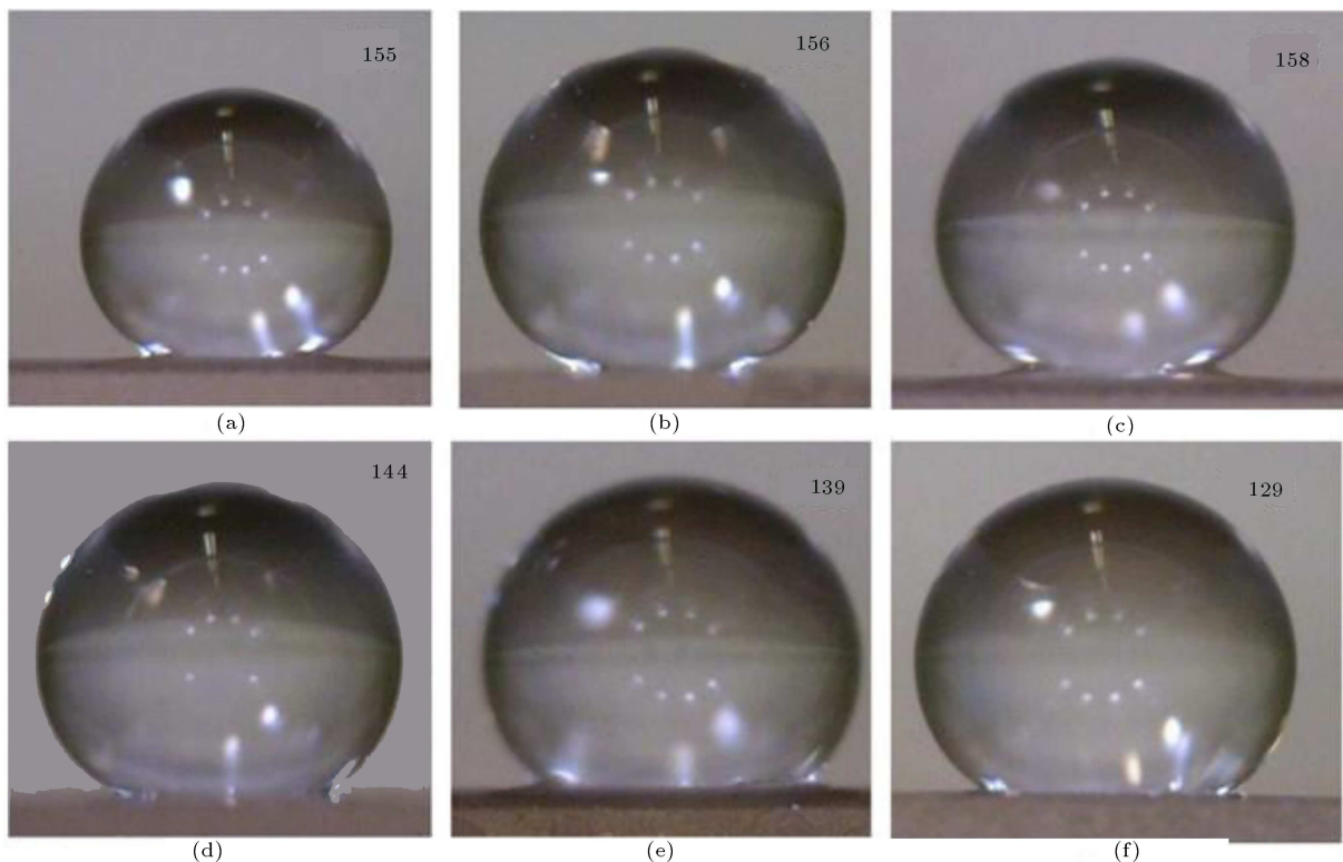
Figure 6. Contact angles of Ni-PTFE composite coatings deposited at different PTFE concentrations in the electrodeposition bath: (a) 5, (b) 10, (c) 15, (d) 20, (e) 30, and (f) 40 g/L.
