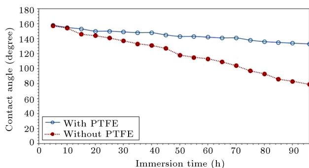
Figure 12. Variation of water contact angle as a function of immersion time for Ni and Ni-PTFE composite coating.
