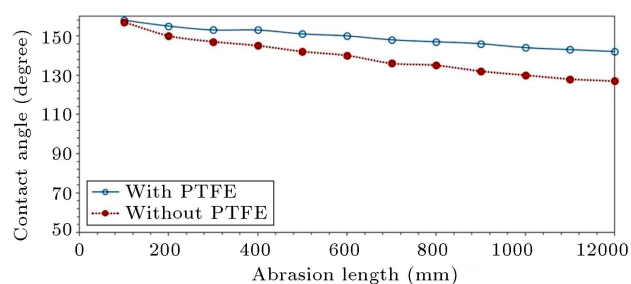
Figure 13. Variation of water contact angle as a function of abrasion length for Ni and Ni-PTFE composite coating.
