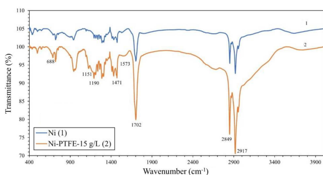
Figure 8. FTIR spectra of Ni coating and Ni-PTFE composite coating deposited at PTFE concentration of 15 g/L in electrodeposition bath.
