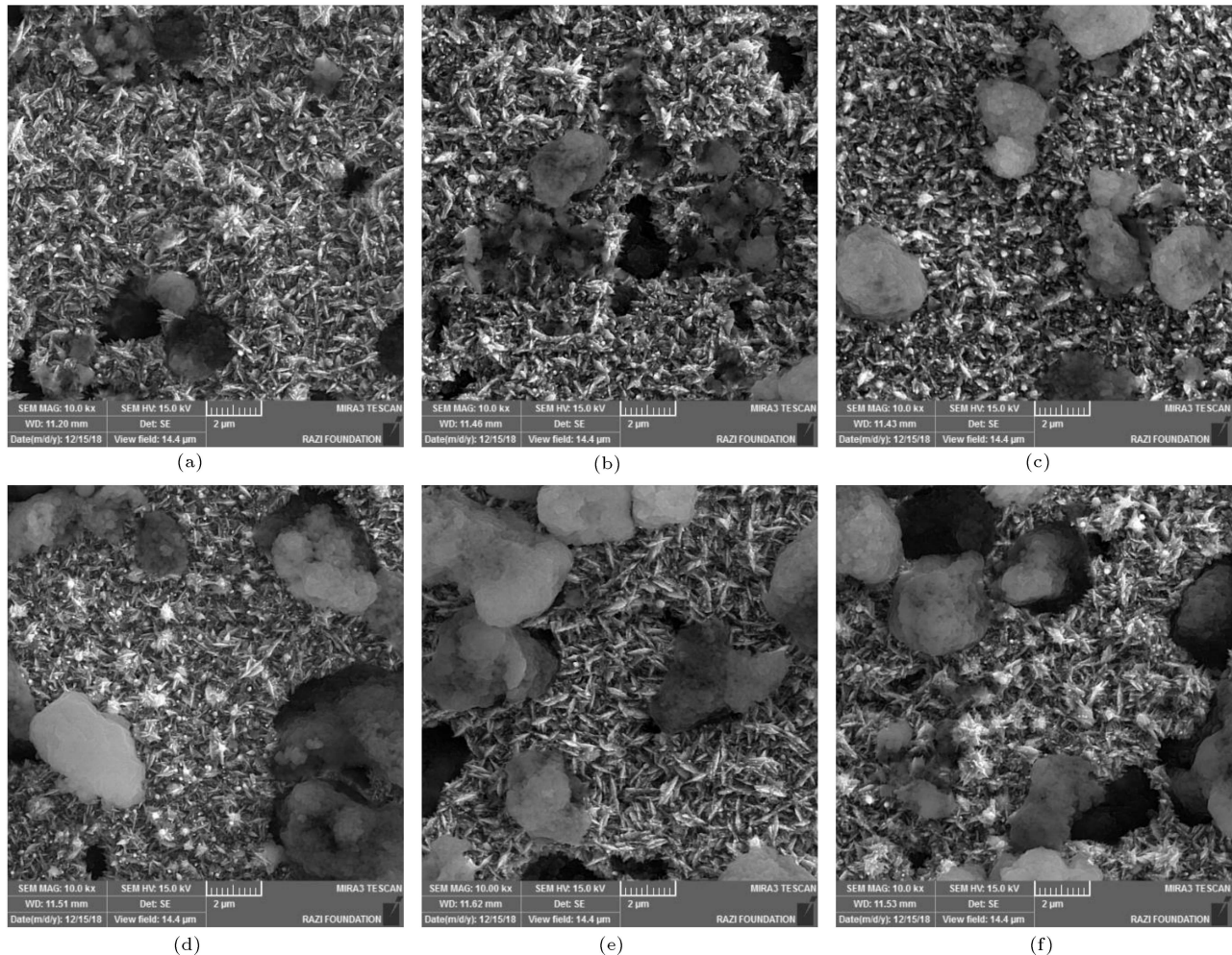
Figure 3. FESEM images of Ni-PTFE coatings fabricated at different PTFE concentrations in electrodeposition bath: (a) 5, (b) 10, (c) 15, (d) 20, (e) 30, and (f) 40 g/L.
