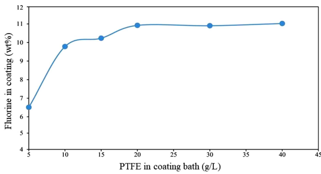
Figure 5. Variation of Fluorine in the Ni-PTFE coating as a function of PTFE in the deposition bath.
