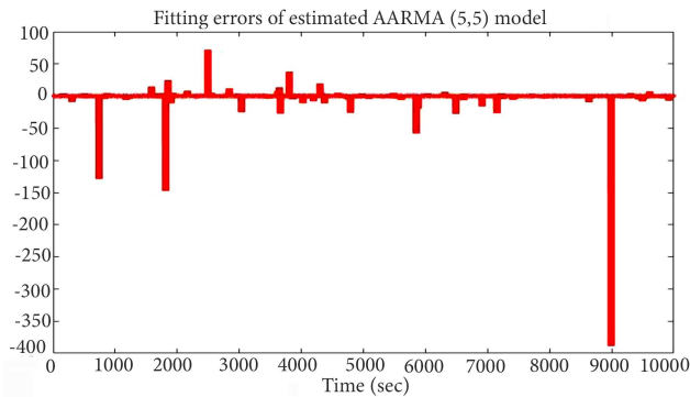
Figure 7. Fitting errors of estimation using AARMA (5, 5).
