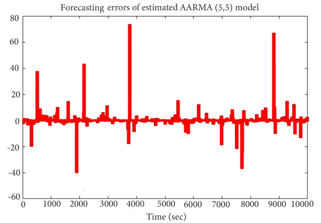
Figure 8. Forecasting errors of estimation using AARMA (5, 5).
