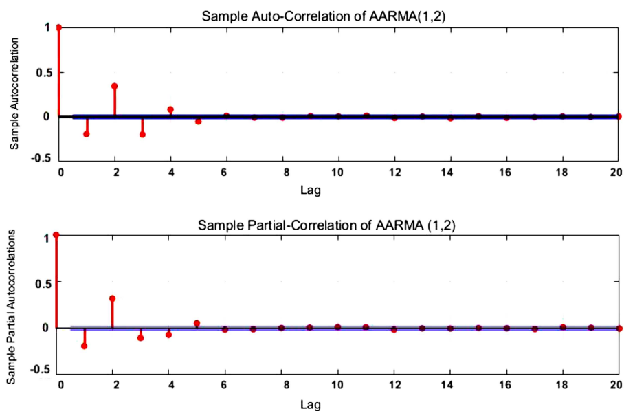
Figure 4. Auto-correlation for the time series used in AARMA.
