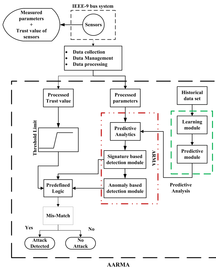
Figure 3. Proposed AARMA model.
