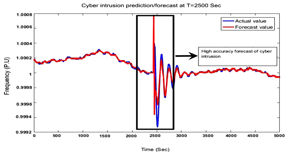
Figure 9. Cyber intrusion forecasting at Bus no. 7 in terms of frequency (Case I).
