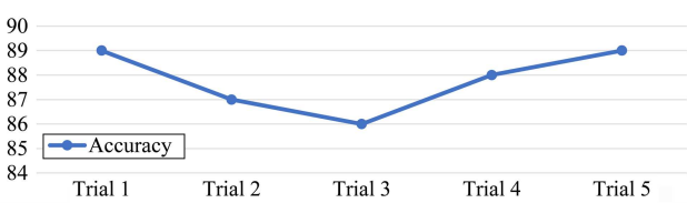
Figure 15. Accuracy for the IEEE 33-bus test system.
