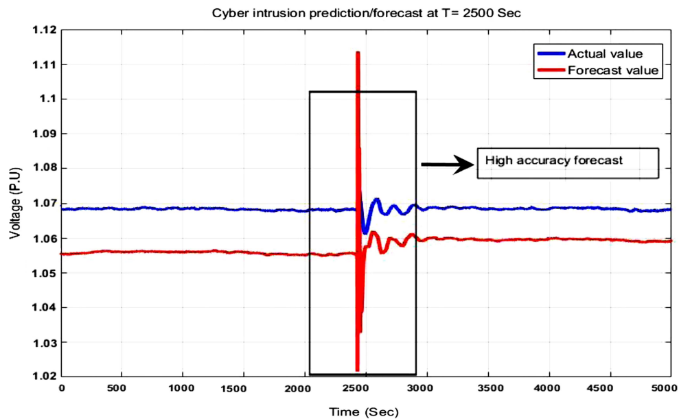
Figure 10. Cyber intrusion forecasting at Bus no. 7 in terms of voltage (Case I).
