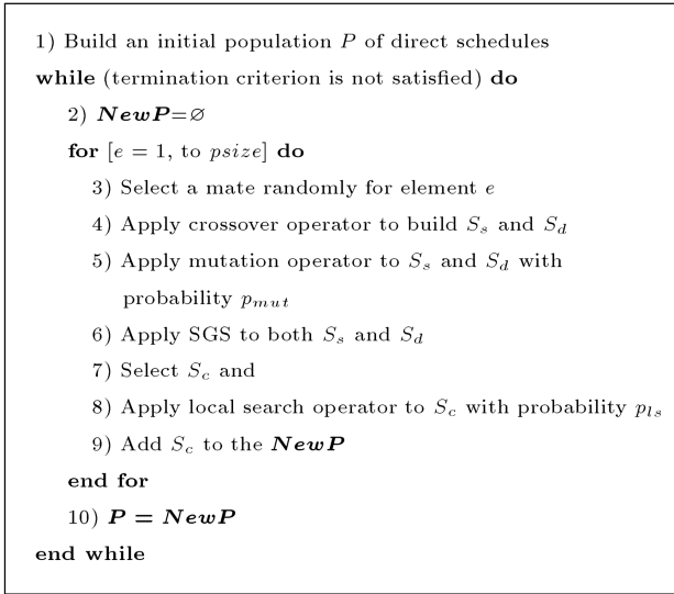
Figure 8. General structure of GA.
