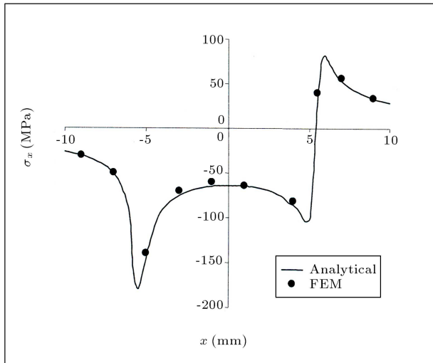
Figure 6. \sigma_x in the depth of 0.1 mm in the sample model.
