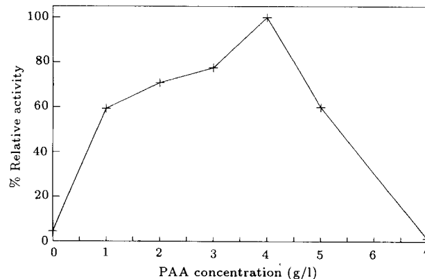
Figure 7. The effect of phenyl acetic acid concentration ( \text{g.l}^{-1} ) on the relative activity of penicillin G acylase (%).
