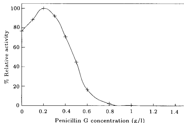
Figure 8. The effect of penicillin G concentration ( \text{g.l}^{-1} ) on the relative activity of penicillin G acylase (%).
